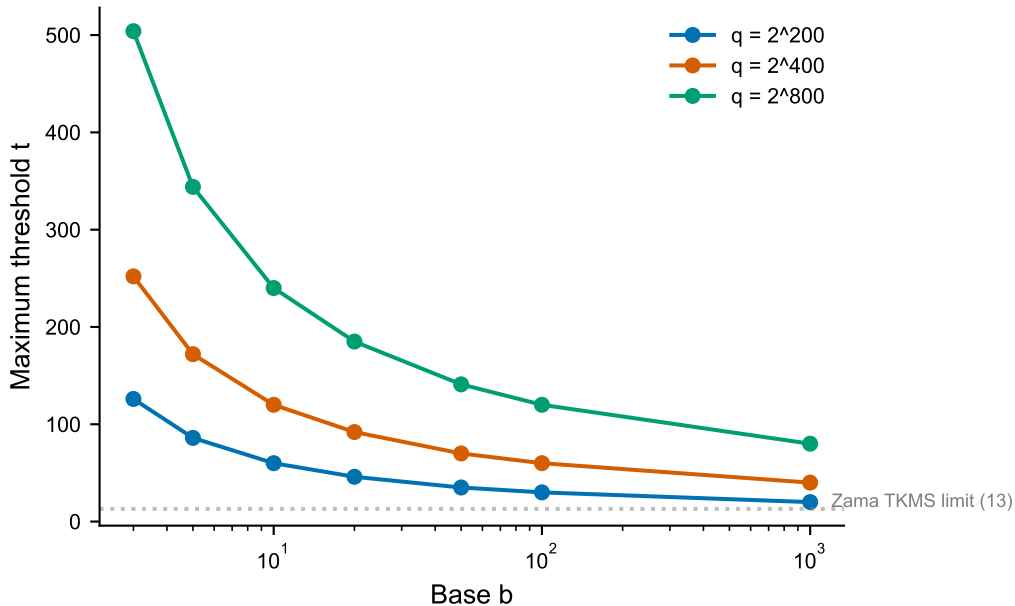
Maximum parties vs base b for different FHE moduli
