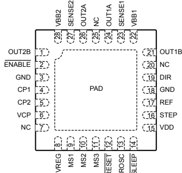
Pinout Diagram
