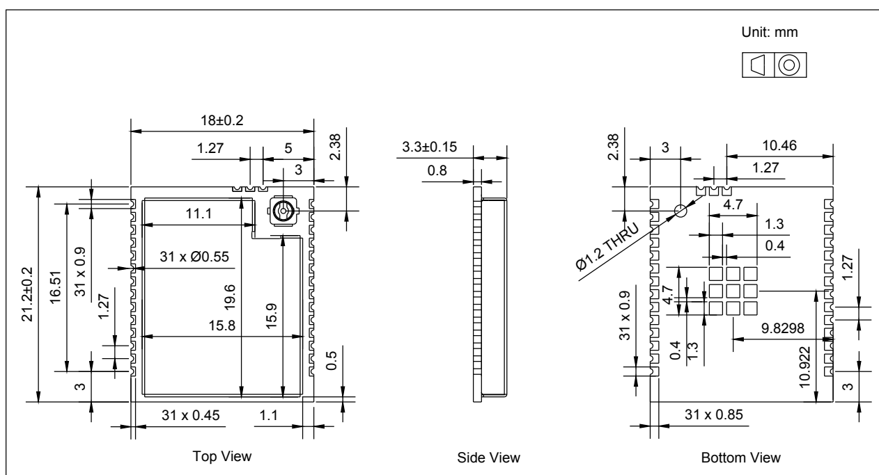
Figure 10-2. ESP32-C5-WROOM-1U Dimensions
