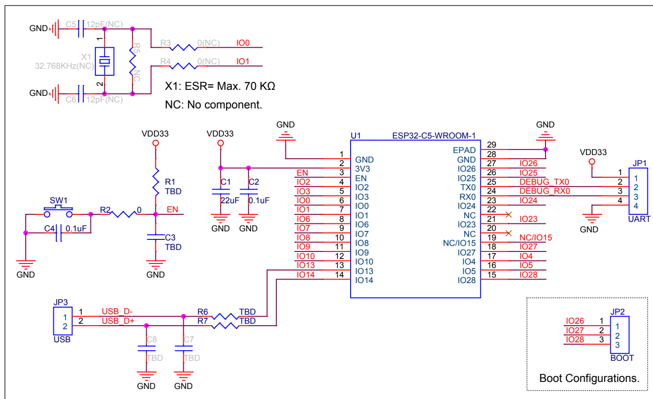
Figure 9-1. ESP32-C5-WROOM-1 Schematics
