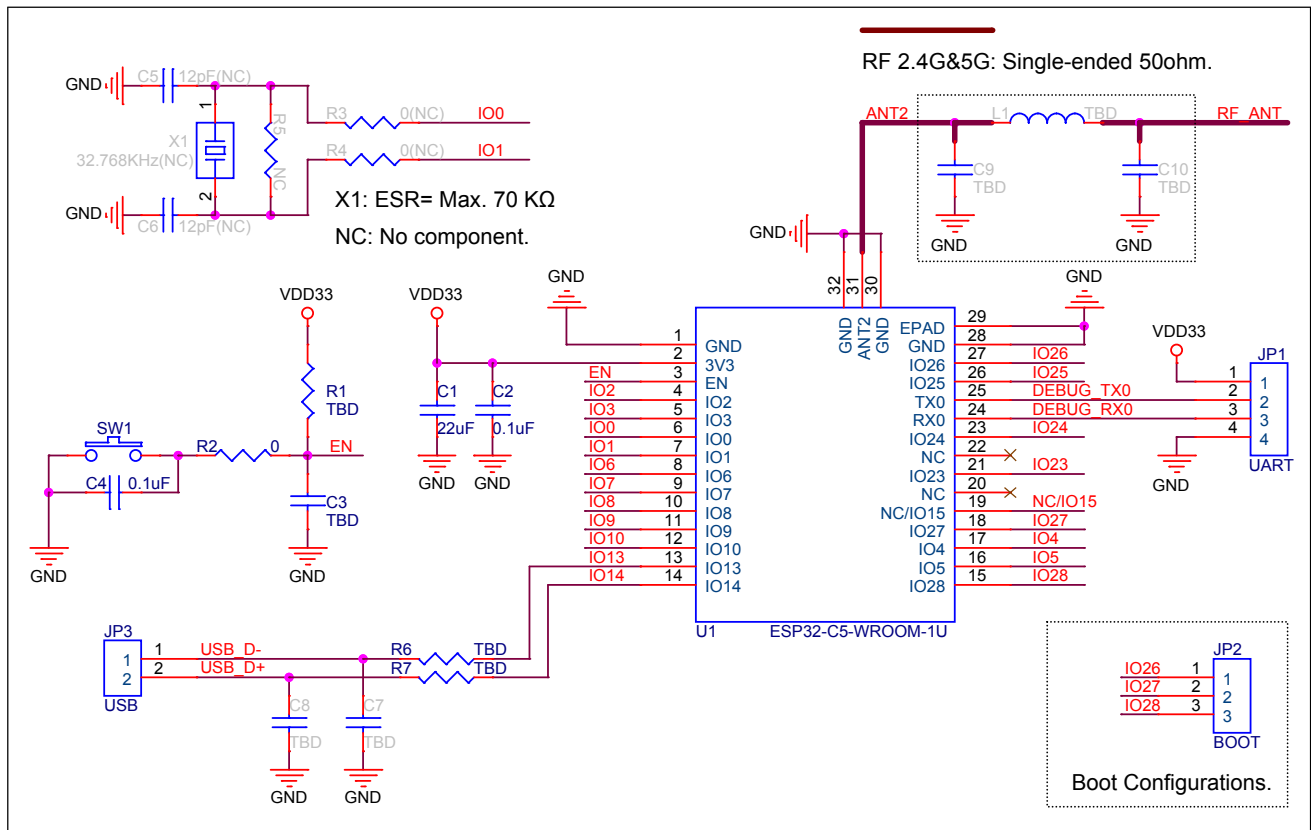
Figure 9-2. ESP32-C5-WROOM-1U Schematics
