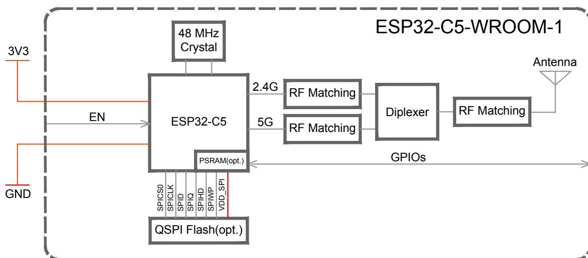
Figure 2-1. ESP32-C5-WROOM-1 Block Diagram
