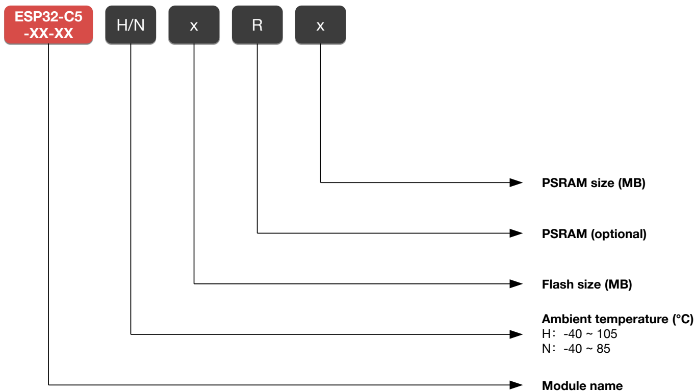
Figure 1-1. ESP32-C5 Module Variant Nomenclature
