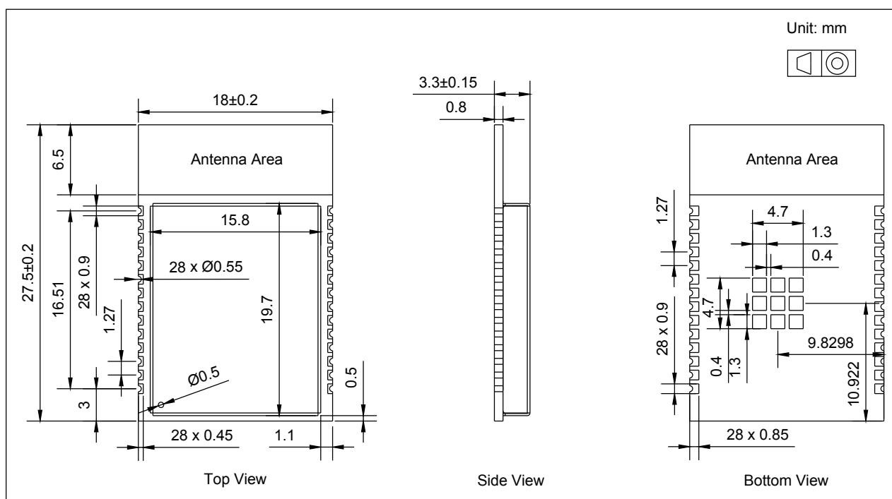
Figure 10-1. ESP32-C5-WROOM-1 Dimensions
