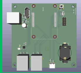
PCB render
