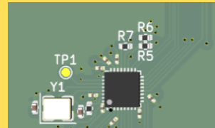
RTL8111H controller
