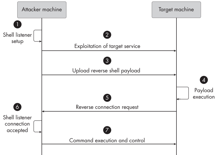
Figure 7-1: The communication sequence of a reverse shell
