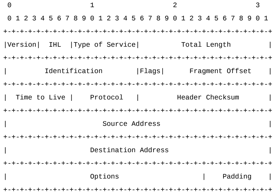
Example Internet Datagram Header
