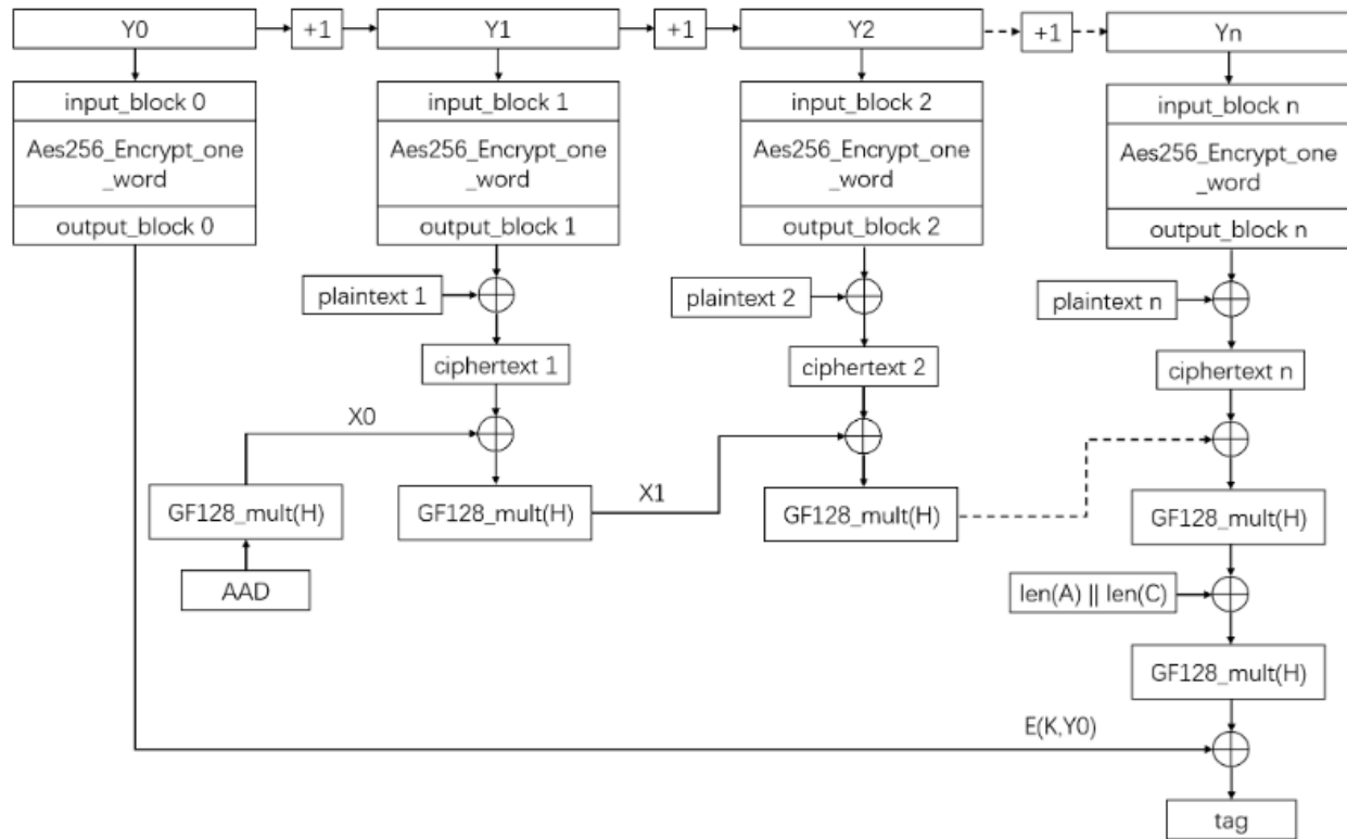
Gambar 1.2.2 AES-GCM
