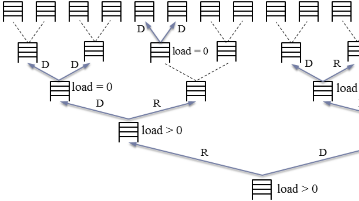
Figure 1: The Evict algorithm. Upon every data access operation, two buckets are chosen at every level of the tree for eviction during which one data block will be evicted to one of its children. To ensure security, a dummy eviction is performed for the child that does not receive a block; further, if the bucket chosen for eviction is empty, dummy evictions are performed on both child buckets. In this figure, R denotes a real eviction and D denotes a dummy eviction.
