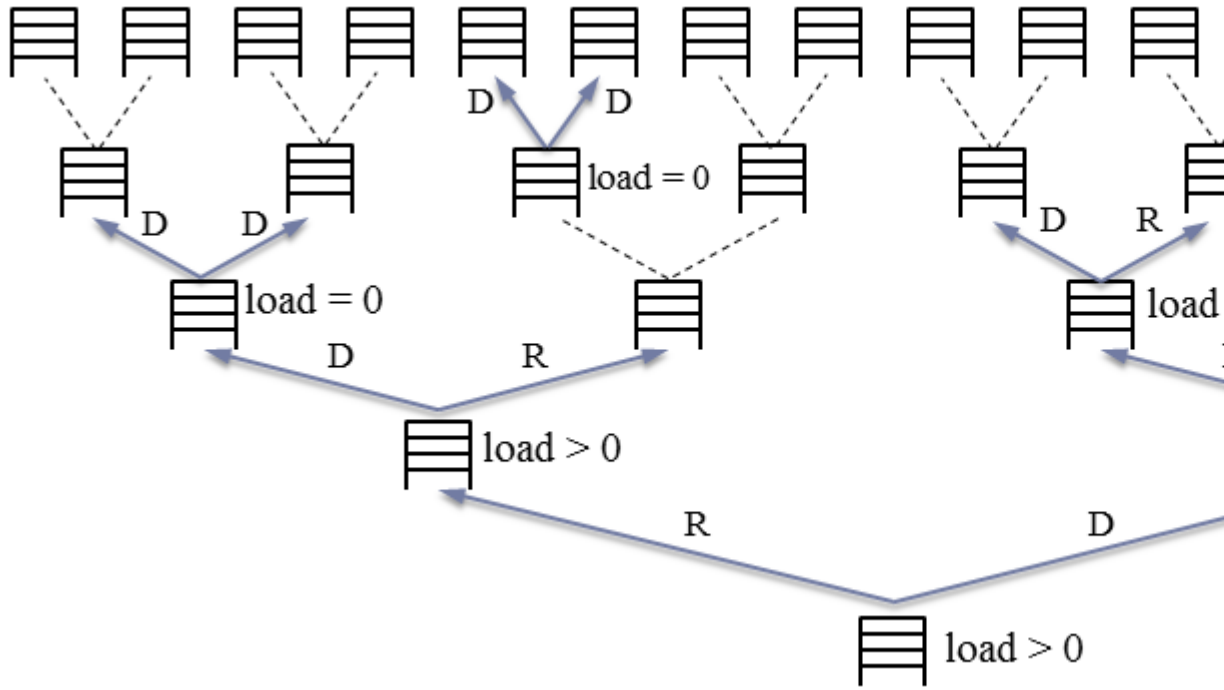
Figure 1: The Evict algorithm. Upon every data access operation, two buckets are chosen at every level of the tree for eviction during which one data block will be evicted to one of its children. To ensure security, a dummy eviction is performed for the child that does not receive a block; further, if the bucket chosen for eviction is empty, dummy evictions are performed on both child buckets. In this figure, R denotes a real eviction and D denotes a dummy eviction.
