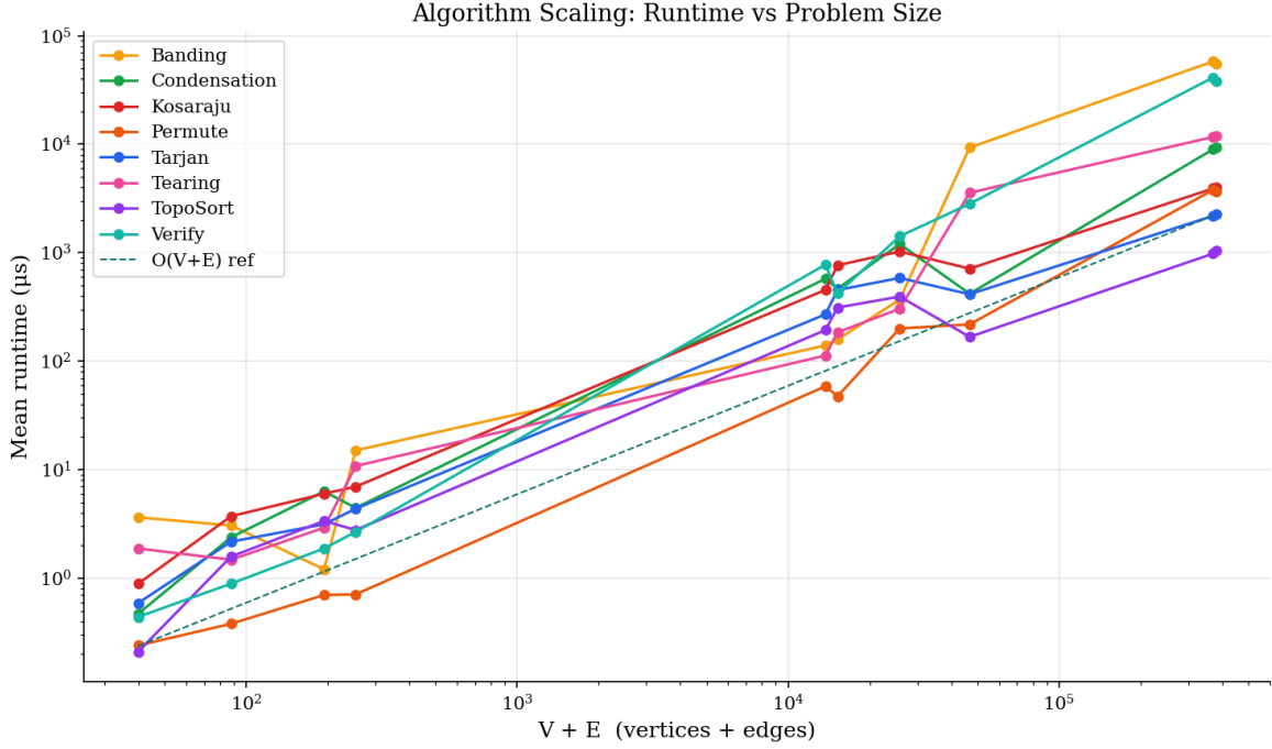
Figure 3: Log-log runtime scaling versus problem size ( V + E ) for benchmarked algorithms.
