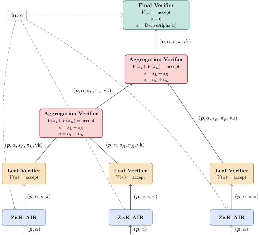
FIGURE 5. Example aggregation tree (binary, unbalanced). Dashed arrows carry the program-level challenge \alpha down to the leaves. Solid arrows carry inputs and outputs to each level: each node's outgoing label is its output, and the incoming labels at any node are its inputs.
