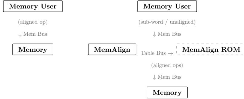
FIGURE 2. Memory access paths. Aligned 8-byte operations go directly to Memory; sub-word and unaligned operations are first decomposed by MemAlign into aligned 8-byte operations.
