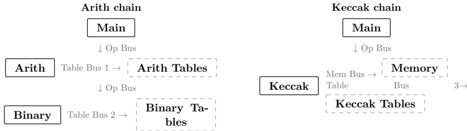
FIGURE 1. Two example chip dependency chains in ZisK. Solid borders denote instruction executor chips; dashed borders denote table chips. Left: the Main chip dispatches an arithmetic operation to Arith via the Operation Bus; Arith queries its own tables and further delegates to Binary, which queries its own tables. Right: Main dispatches a cryptographic operation to Keccak; the precompile simultaneously reads its inputs and writes its outputs via the Memory Bus and queries its own tables. In both cases each chip proves only its own local constraints, and bus balancing composes the arguments into a global proof.
