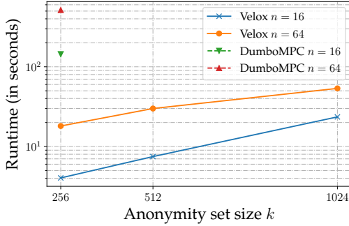
Figure 2: Anonymity set size k vs Runtime: We plot the runtime of Velox and DumboMPC’s OptRanTriGen protocol at n = 16, 64 parties. Velox is 36 \times faster n = 16 and 28.6 \times faster than DumboMPC at n = 64 for k = 256 . We were unable to successfully run DumboMPC for higher values of k .
