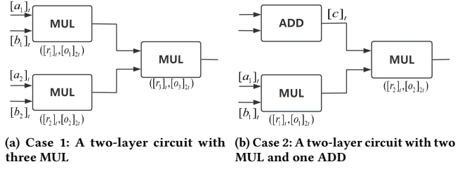
Figure 6: Two Cases for a two-layer circuit with three gates. Here [o]_{2t} is a degree- 2t Shamir sharing of 0 and we use it to replace [r]_{2t} in the double sharing , this is the observation in [GLO + 21] which helps to decouple the relation between degree- t and 2t sharings.
