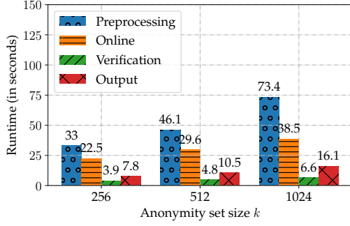
Figure 4: Phase-wise runtime in a geo-distributed testbed: We plot a phase-wise latency of Velox running with n = 112 parties mixing a batch of k = 256, 512, 1024 messages. The pre-processing phase, where parties generate random sharings, is the most expensive phase of all. In this setting with a high round trip time, the online phase contributes a substantial latency to the overall runtime, mainly because of its round complexity.
