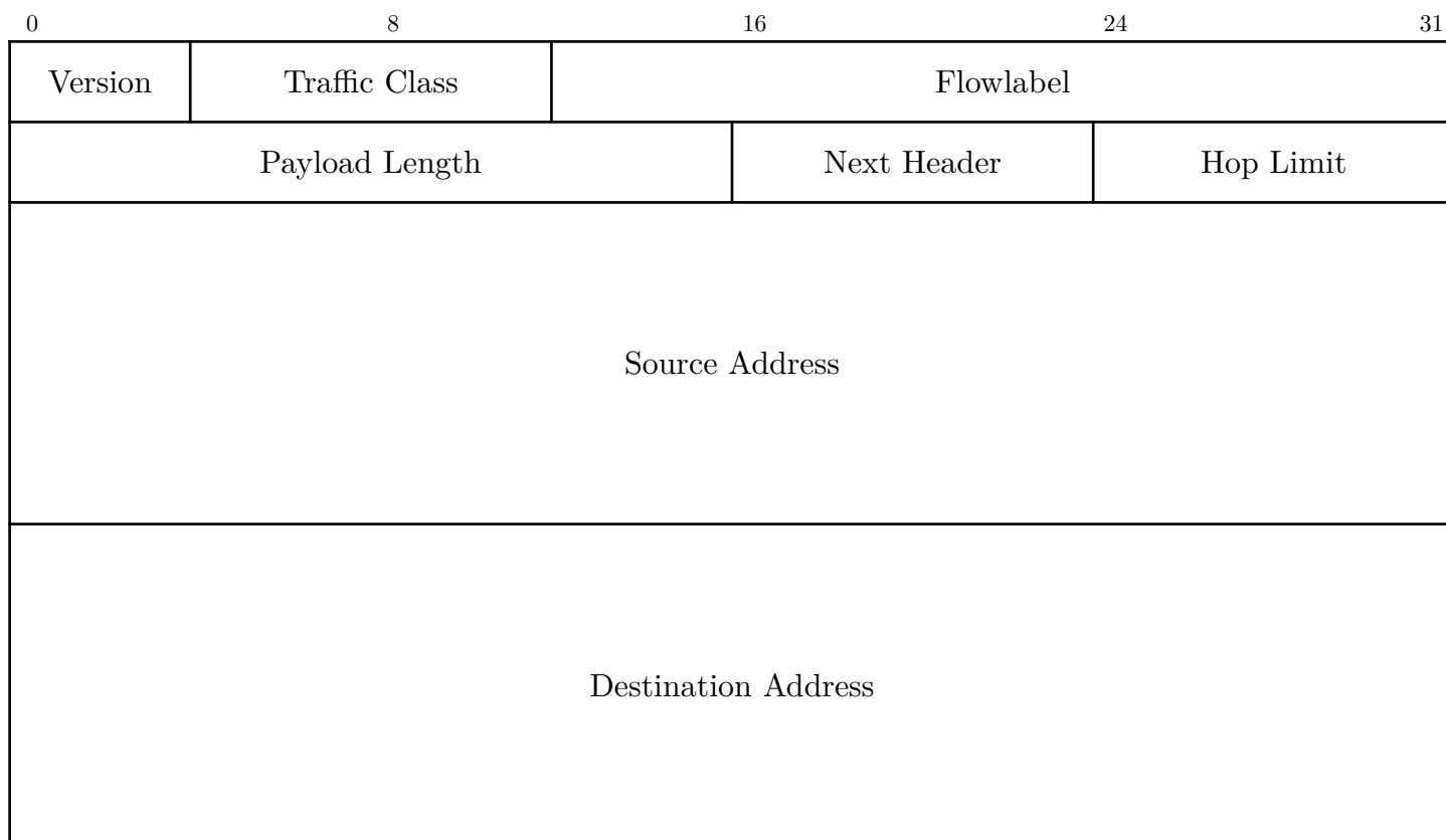
Figure 2: Struktura IPv6 packetu
