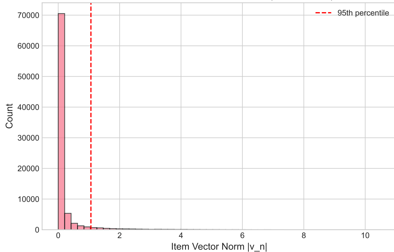
Distribution of Item Vector Norms (Polarization)
