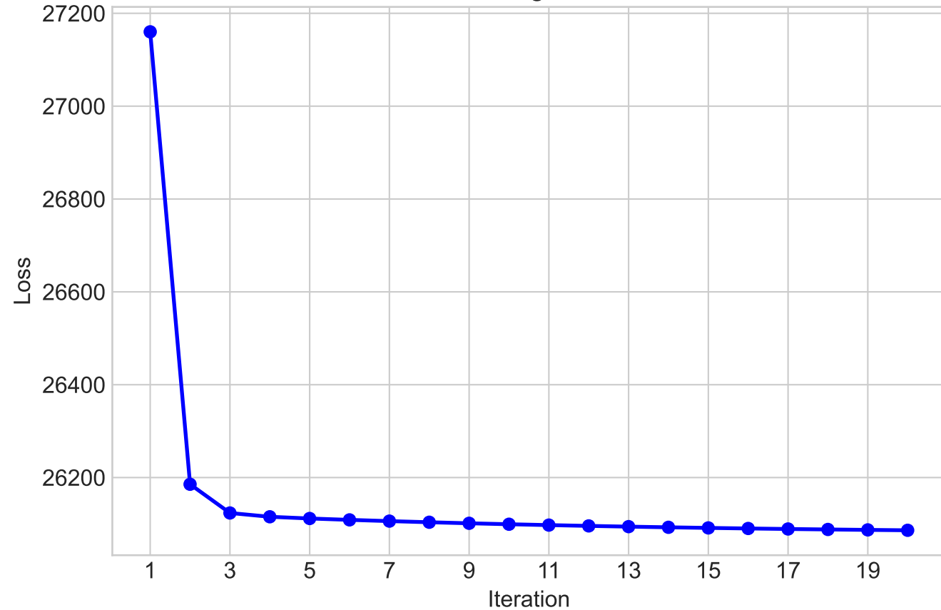
Training Loss
