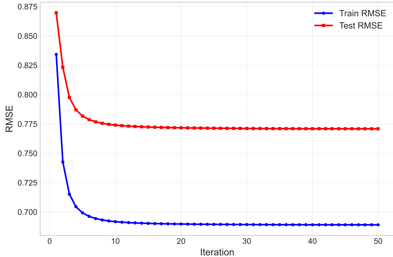
Learning Curves: Train vs Test RMSE
