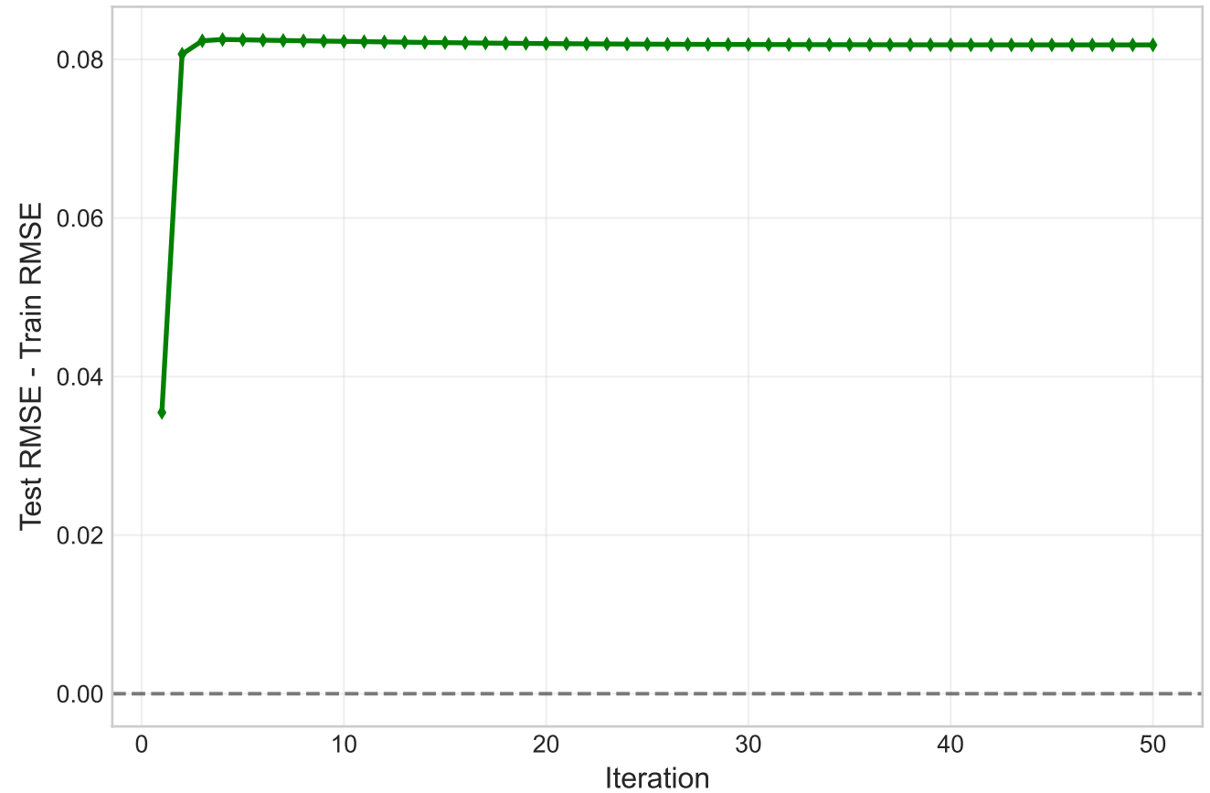
Generalization Gap (Overfitting Indicator)
