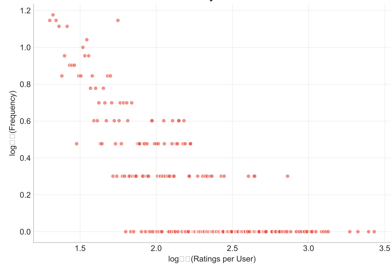
User Activity Power Law
