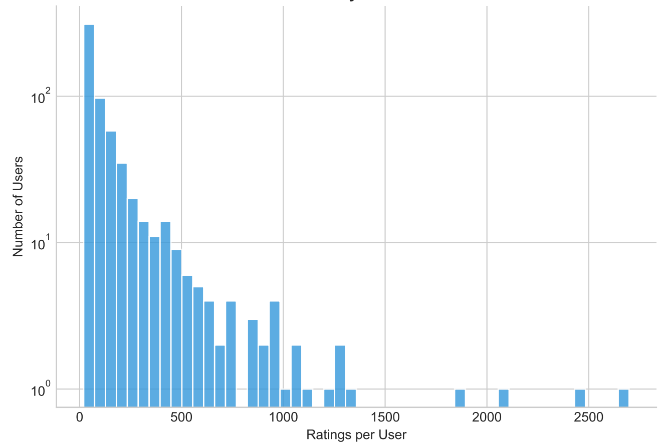
User Activity Power Law
