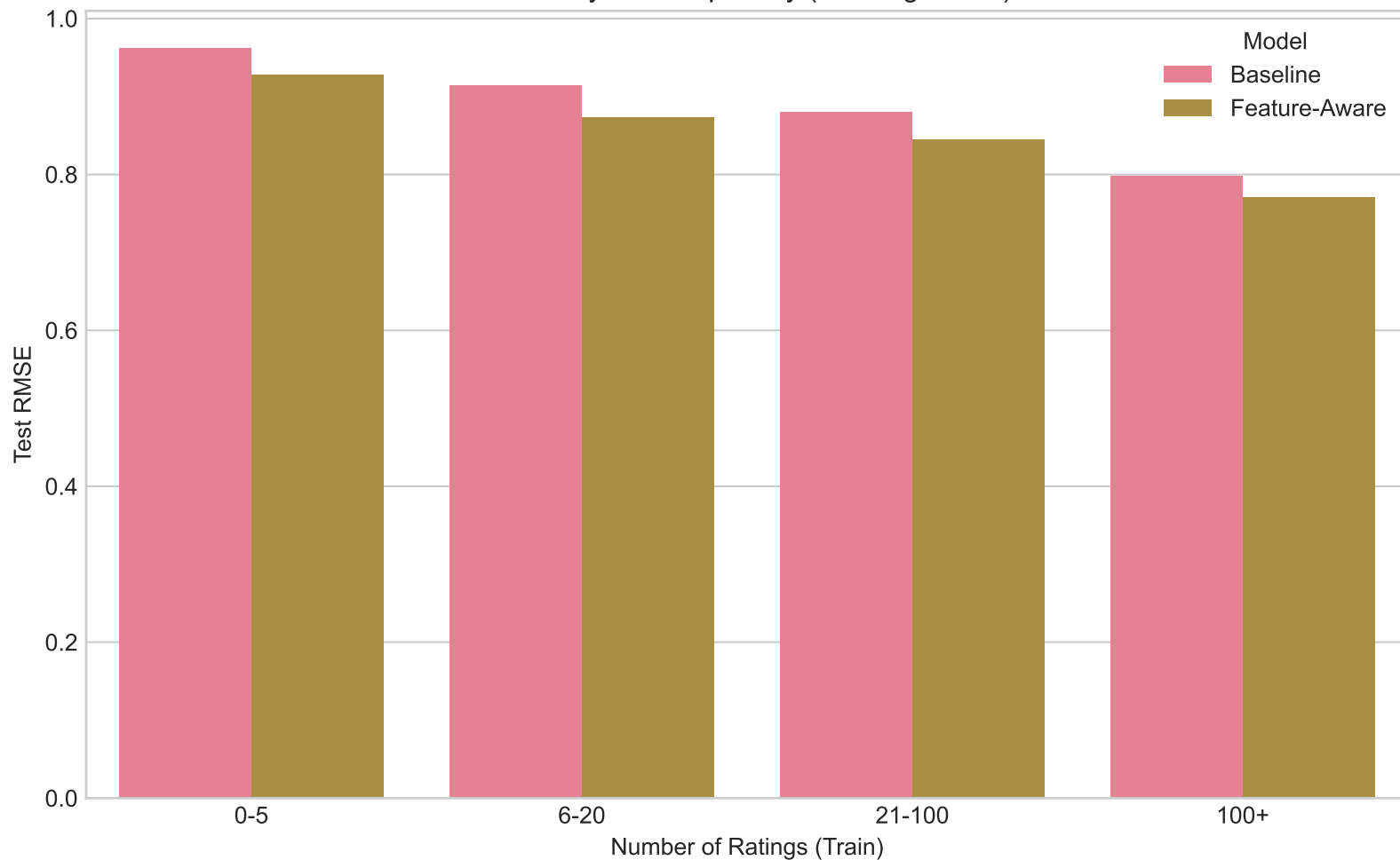
RMSE by Item Popularity (Training Count)
