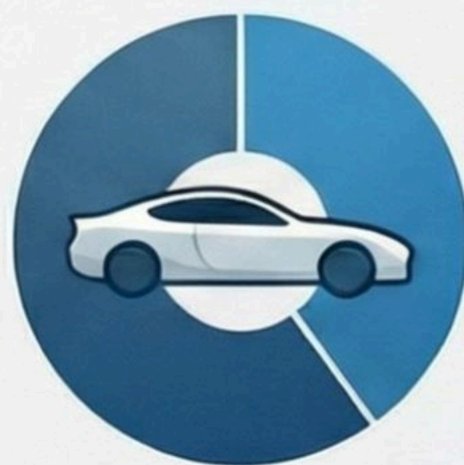
Automotive Industry | 40%
