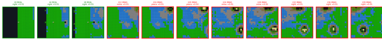
Figure 6: A DREAMERV3 imagined rollout decoded to sprites (green border = real warmup, red = open-loop imagination). The world model imagines coherent terrain — including the edge tree bands — and dreams mining/placing through the middle.
