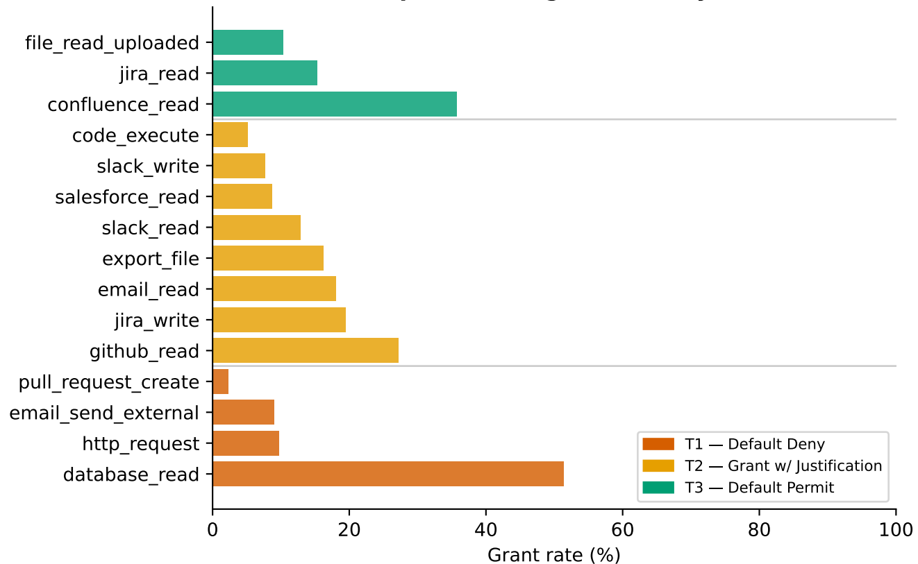
LLM permission grant rate by tool
