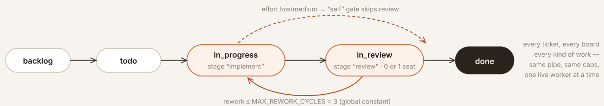
Fig. 2 — the compiled-in lifecycle. The only per-task levers are which models sit in each of two seats and an effort knob that doubles, implicitly, as the review-gate switch.
