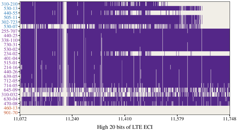
(a) eNodeB-ID occupancy
