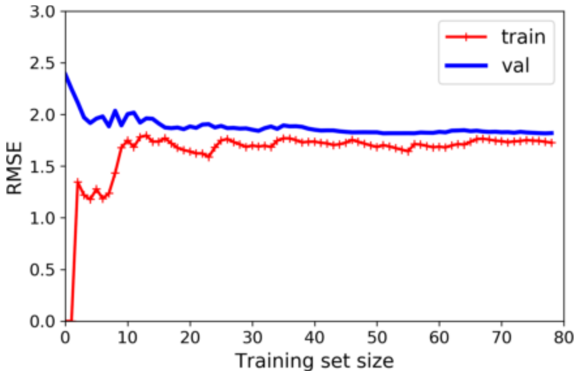
Figure 4-15. Learning curves
