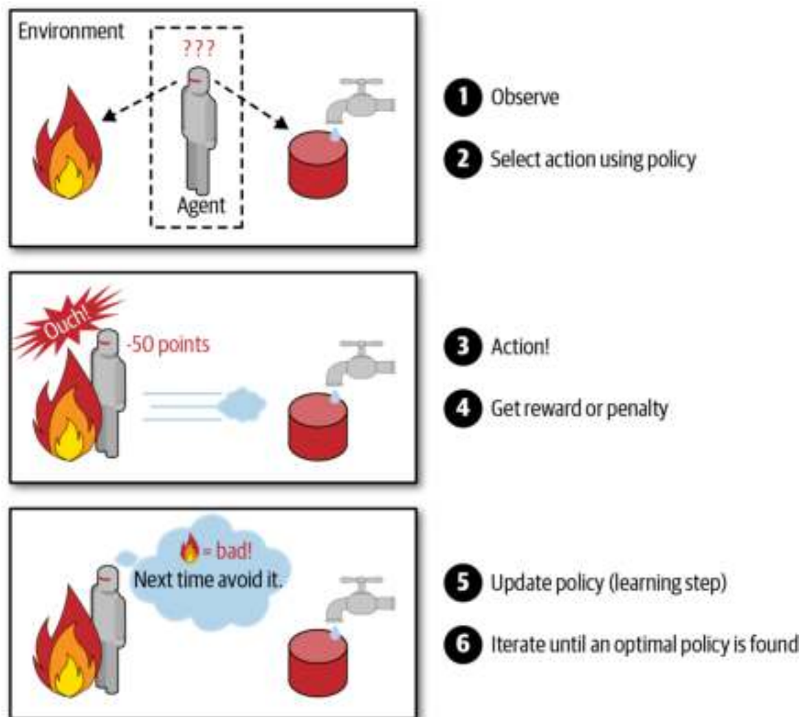
Figure 1-12. Reinforcement Learning
