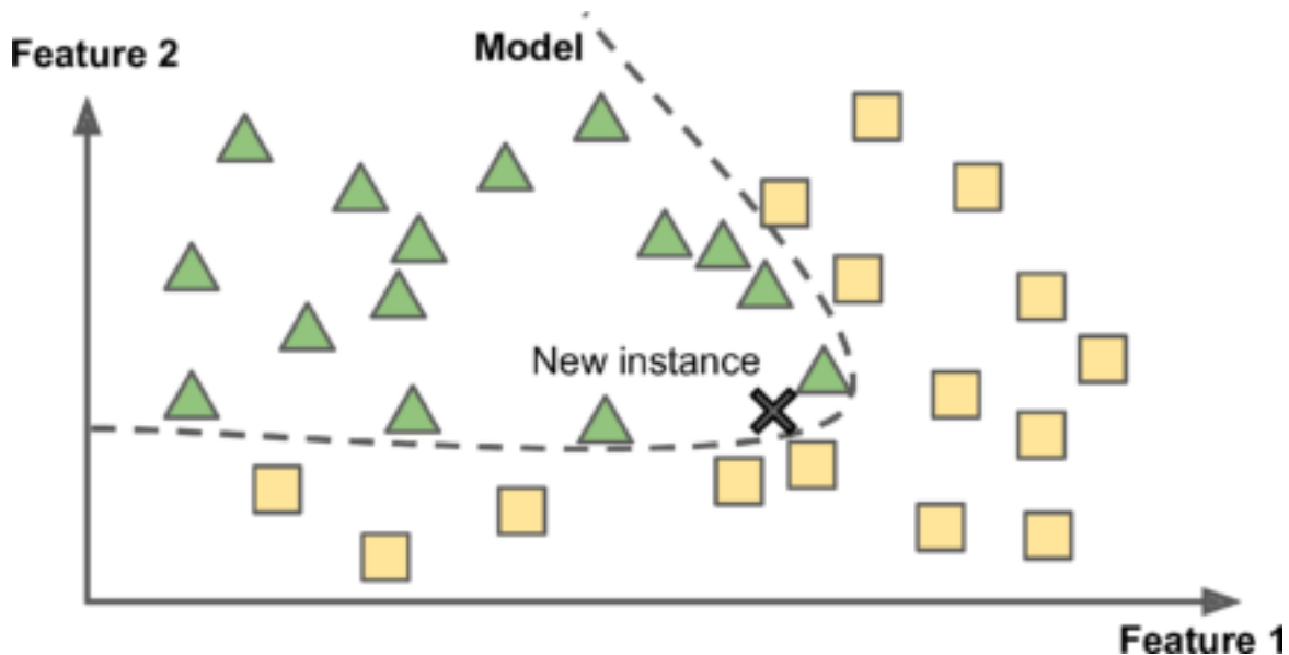
Figure 1-16. Model-based learning
