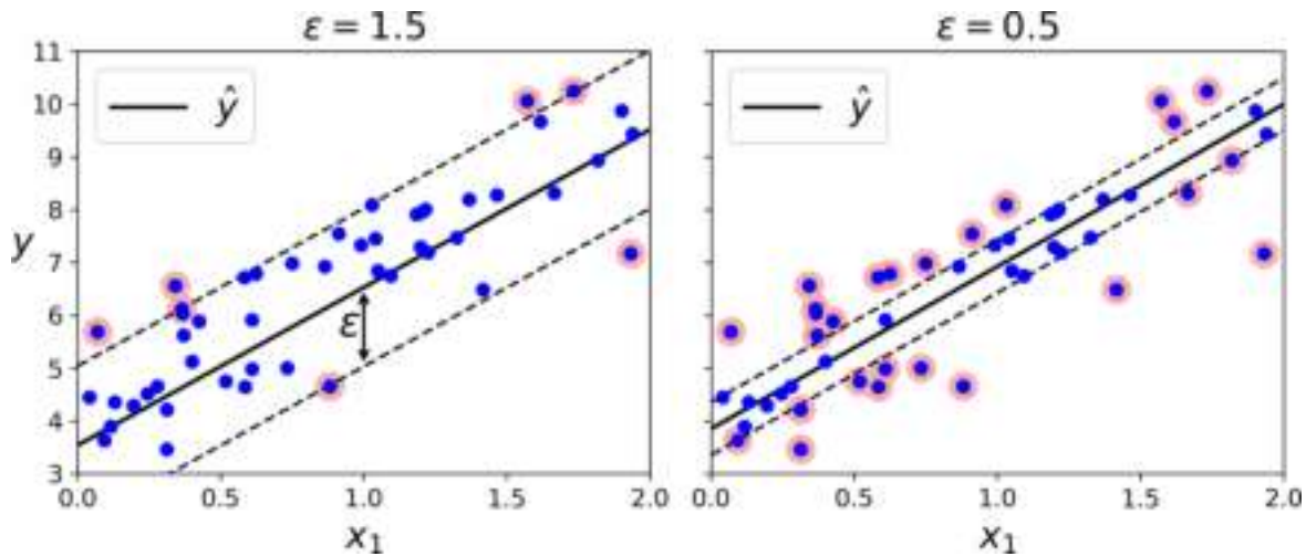
Figure 5-10. SVM Regression
