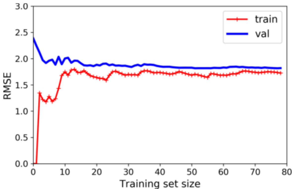
Figure 4-15. Learning curves
