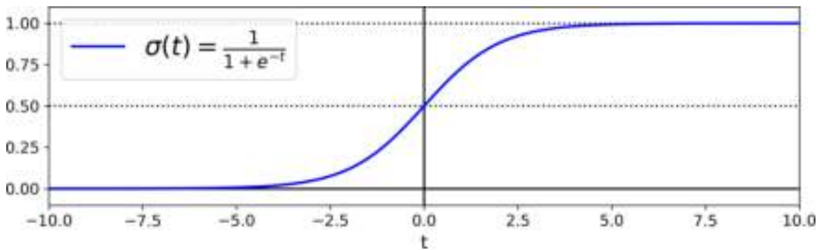
Figure 4-21. Logistic function
