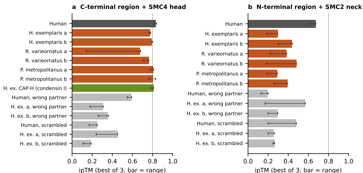
Figure 4: Predicted binding of the CAP-H2 regions to the condensin ring. Interface confidence (ipTM) of Boltz-2 predictions, best of three samples; bars show the range across samples. (a) CAP-H2 C-terminal regions with the same species' SMC4 head, the H. exemplaris condensin I kleisin CAP-H with SMC4 (green), and controls: the region offered SMC2 instead (wrong partner) or with its residues shuffled (grey). (b) CAP-H2 N-terminal regions with the SMC2 head and neck, and the same controls. The dotted line marks 0.8, above which predicted interfaces are usually correct.
