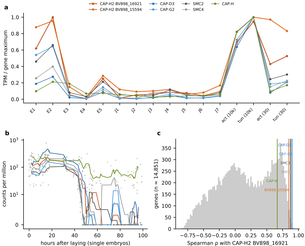
Figure 4: Expression of the H. exemplaris condensin genes. (a) Mean TPM per condition in Yoshida et al. 2017, scaled to each gene’s maximum. E1–E5: egg days; J1–J7: juvenile days; act and tun: active and dried adults, in two sample sizes (10k and 30 animals). (b) Counts per million in 62 single embryos (Levin et al. 2016) against hours after laying; lines are 5-embryo running means. BV898_15594 has no transcript in this assembly. (c) Spearman correlation of CAP-H2 BV898_16921 with every expressed gene across the 48 Yoshida samples; vertical lines mark the condensin subunits.
