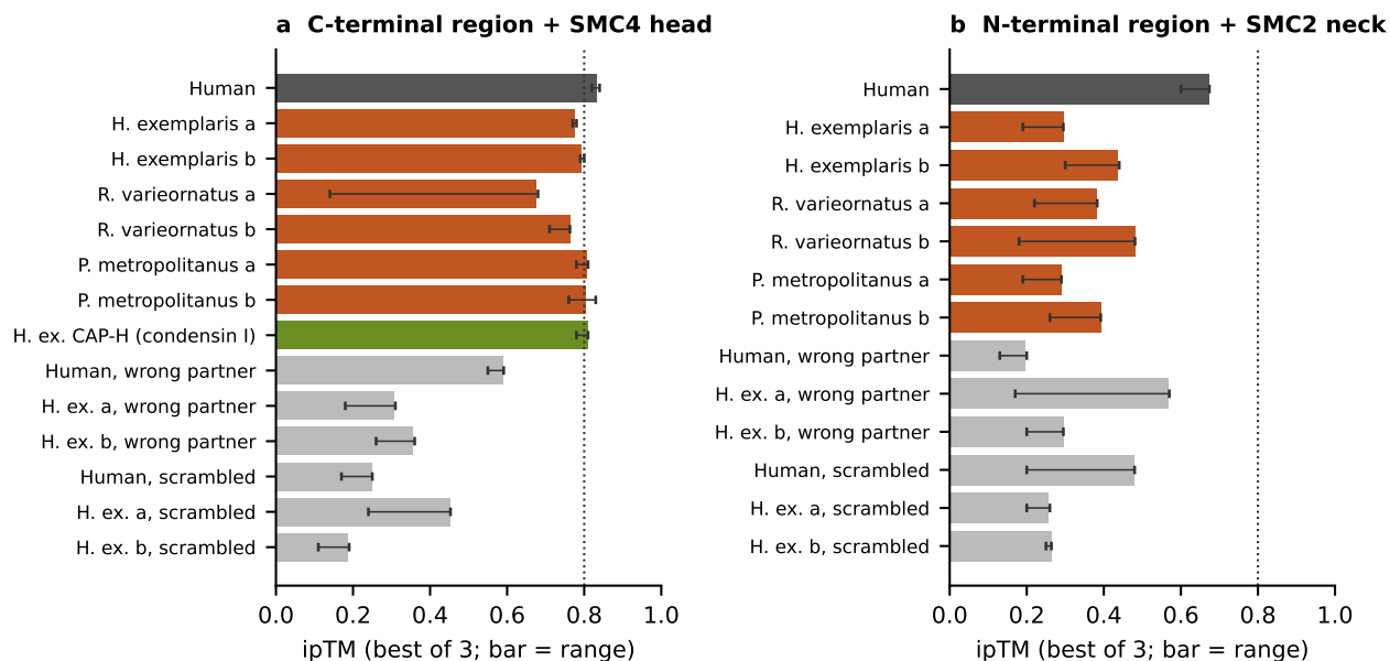
Figure 3: Predicted binding of the CAP-H2 regions to the condensin ring. Interface confidence (ipTM) of Boltz-2 predictions, best of three samples; bars show the range across samples. (a) CAP-H2 C-terminal regions with the same species' SMC4 head, the H. exemplaris condensin I kleisin CAP-H with SMC4 (green), and controls: the region offered SMC2 instead (wrong partner) or with its residues shuffled (grey). (b) CAP-H2 N-terminal regions with the SMC2 head and neck, and the same controls. The dotted line marks 0.8, above which predicted interfaces are usually correct.
