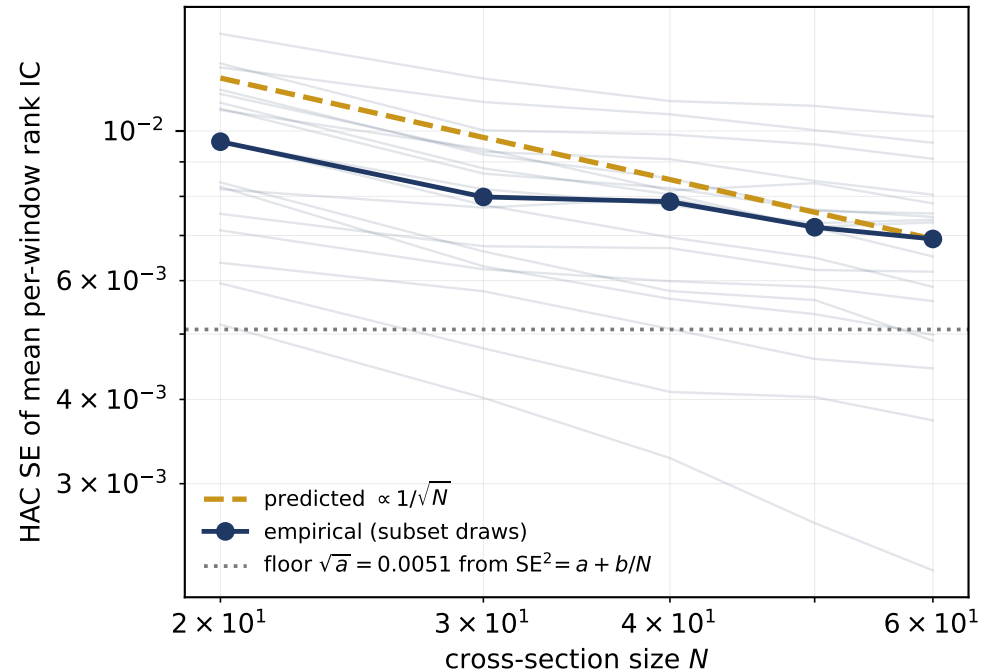
SE scaling: measured N^{-0.29} vs assumed N^{-0.50}
