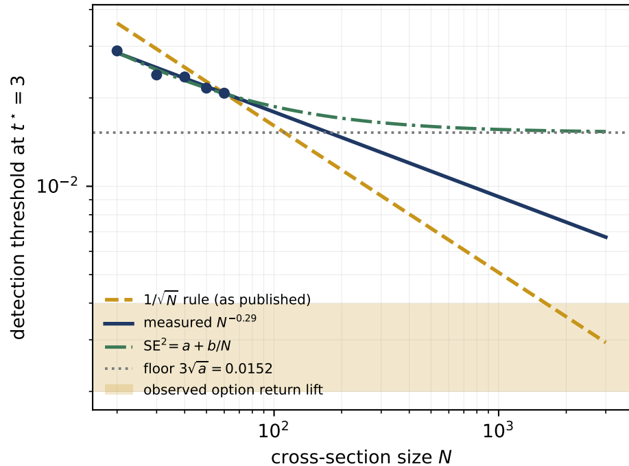
Extrapolated threshold under each scaling law
