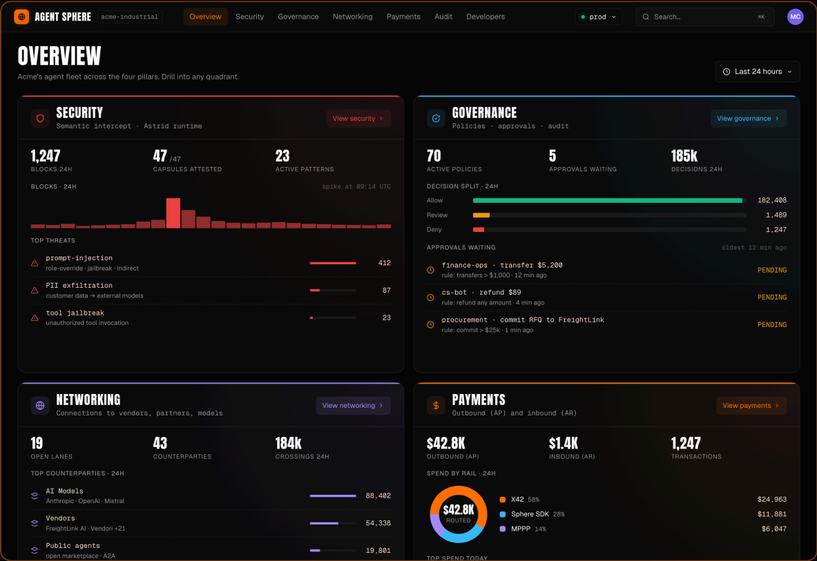
Live: Unicity operator console – one pane of glass across every agent workload.
