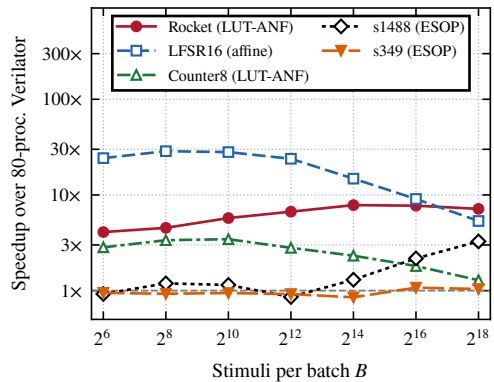
(c) Speedup over the CPU baseline
