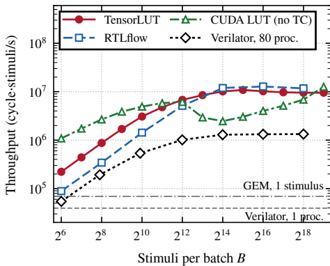
(a) Rocket core throughput
