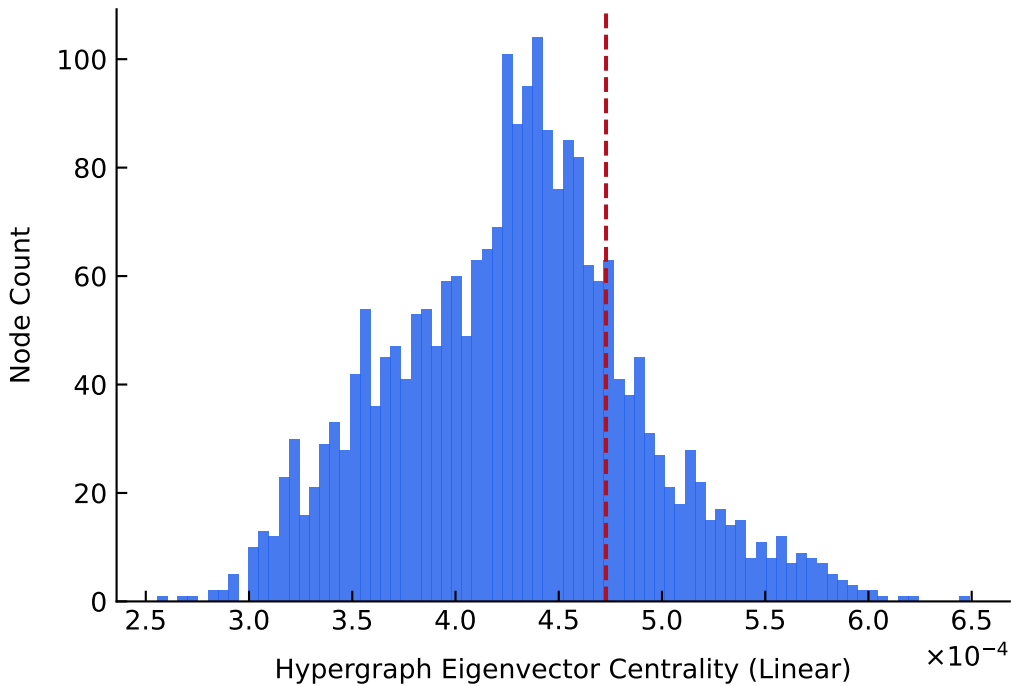
Score Distribution
