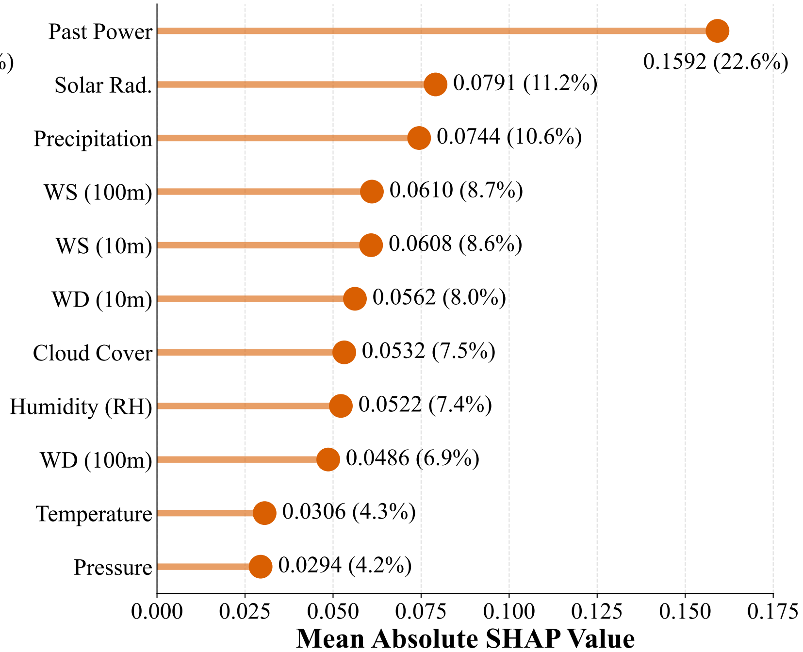
Feature Importance Analysis for Fujian
