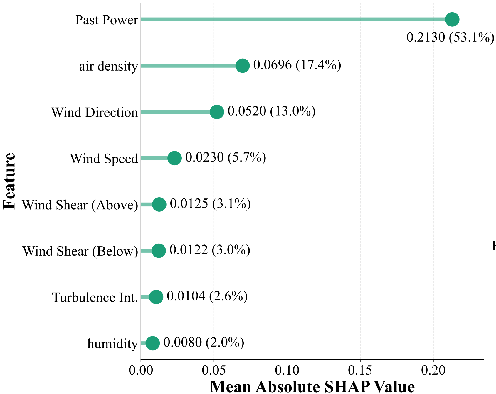
Feature Importance Analysis for DSWE
