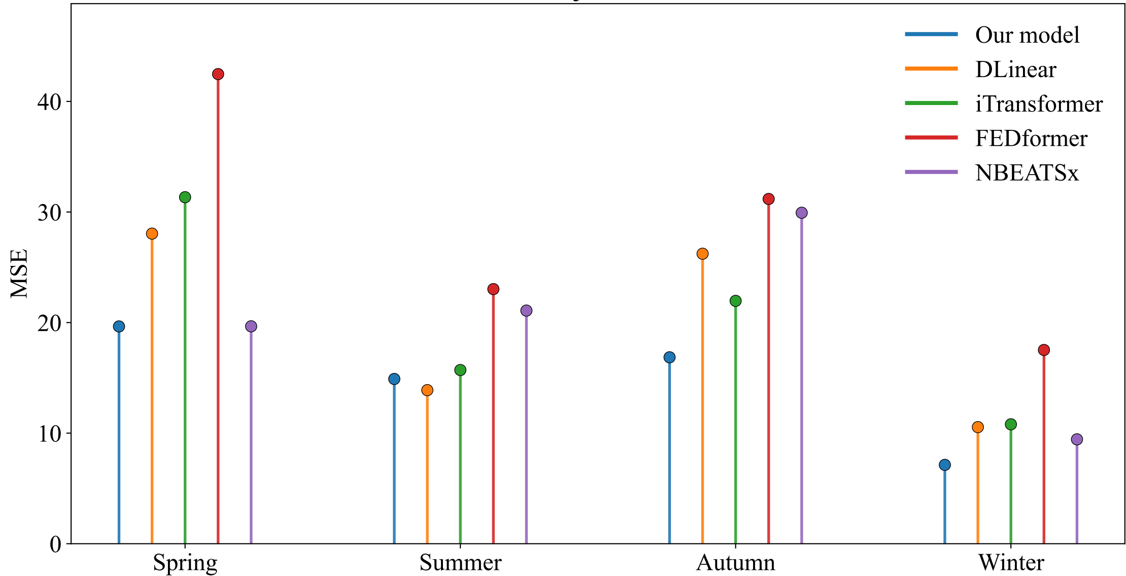
Seasonal MSE Lollipop Chart with Performance Gaps Dataset=fujian, Scale=6-1
