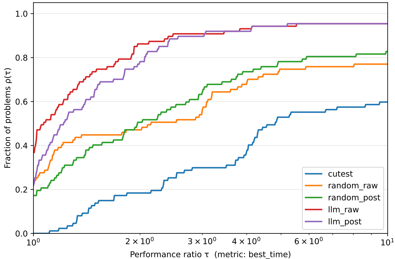
Unbounded — time
