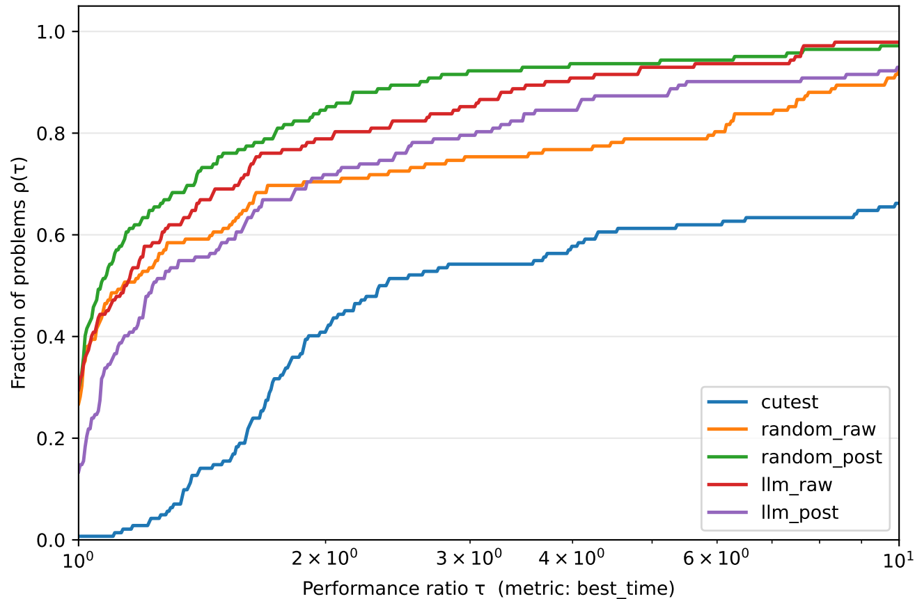
Bounded — time
