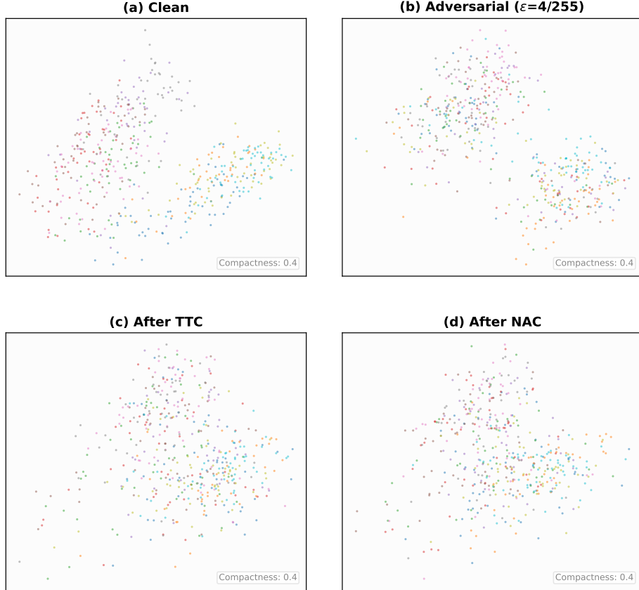
Fig. 4 PCA visualization of CLIP ViT-B/32 embeddings on CIFAR-10 test set. (a) Clean images: well-separated, compact class clusters. (b) Adversarial images ( \epsilon_{\text{att}} = 4/255 ): collapsed and scattered embeddings with severely degraded class structure. (c) After TTC defense: partial restoration of class separation. (d) After NAC defense: more complete restoration, with clusters closer to the clean embedding distribution.
