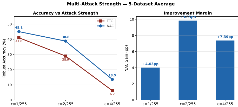
Fig. 3 Multi-attack strength analysis. Left: robust accuracy of TTC and NAC as a function of attack budget. Right: NAC improvement margin. The gain peaks at \epsilon_{\text{att}} = 2/255 and declines at \epsilon_{\text{att}} = 4/255 , consistent with the local smoothness hypothesis.
