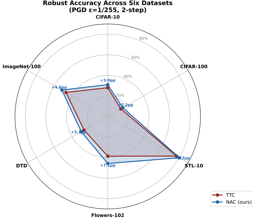
Fig. 2 Radar chart of TTC and NAC robust accuracy across six datasets under PGD \epsilon_{\text{att}} = 1/255 . NAC consistently encloses TTC, with the largest gain on Flowers-102 (+7.14pp).
