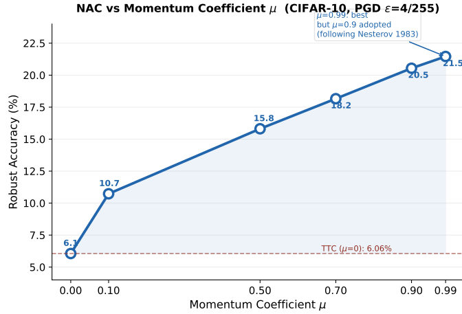
Fig. 5 Robust accuracy of NAC as a function of the momentum coefficient \mu . The monotonic trend confirms that the look-ahead mechanism provides systematic benefit, with the gain saturating near \mu = 0.9 .
