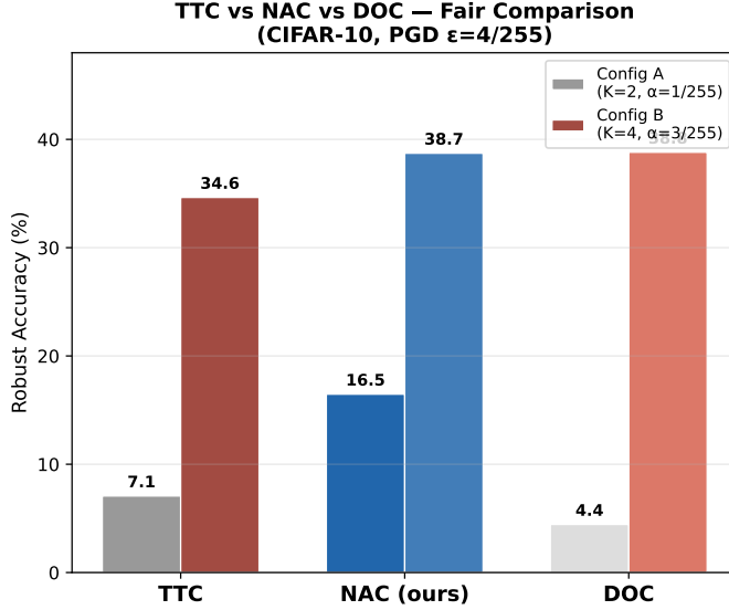
Fig. 6 Grouped comparison of TTC, NAC, and DOC under two configurations. Config A (NAC default: K=2 , \alpha=1/255 ): NAC leads substantially. Config B (DOC default: K=4 , \alpha=3/255 ): NAC and DOC are statistically equivalent, despite DOC’s additional complexity.
