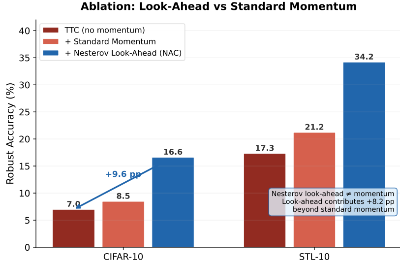
Fig. 4 Ablation comparison of TTC (no momentum), TTC with standard Polyak momentum, and NAC (Nesterov look-ahead). The Nesterov look-ahead contributes substantially more improvement than standard momentum alone, confirming the distinct and complementary nature of the two mechanisms.
