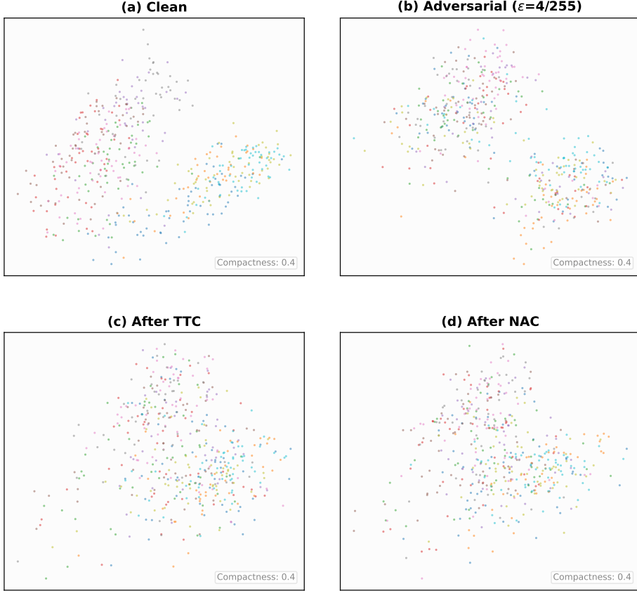
Fig. 7 PCA visualization of CLIP ViT-B/32 embeddings on CIFAR-10 test set. (a) Clean images: well-separated, compact class clusters. (b) Adversarial images ( \epsilon_{\text{att}} = 4/255 ): collapsed and scattered embeddings with severely degraded class structure. (c) After TTC defense: partial restoration of class separation. (d) After NAC defense: more complete restoration, with clusters closer to the clean embedding distribution.
