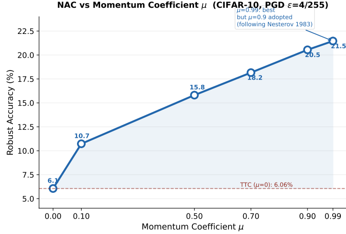
Fig. 3 Robust accuracy of NAC as a function of the momentum coefficient \mu . The monotonic trend confirms that the look-ahead mechanism provides systematic benefit, with the gain saturating near \mu = 0.9 .
