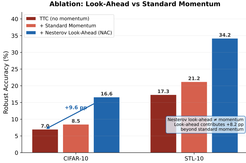
Fig. 2 Ablation comparison of TTC (no momentum), TTC with standard Polyak momentum, and NAC (Nesterov look-ahead). The Nesterov look-ahead contributes substantially more improvement than standard momentum alone, confirming the distinct and complementary nature of the two mechanisms.
