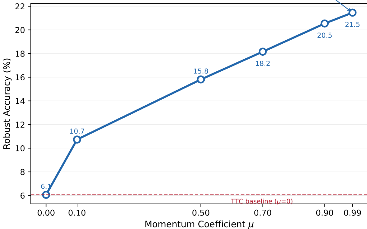
NAC Performance vs Momentum Coefficient \mu (CIFAR-10, PGD \epsilon=4/255 )
