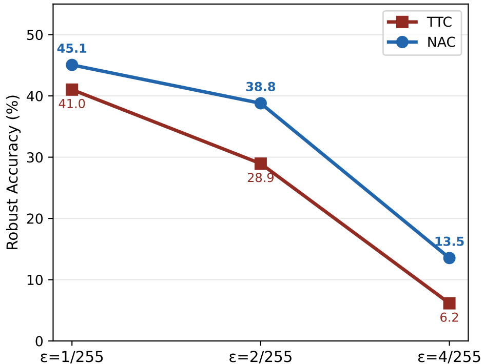
Accuracy vs Attack Strength
