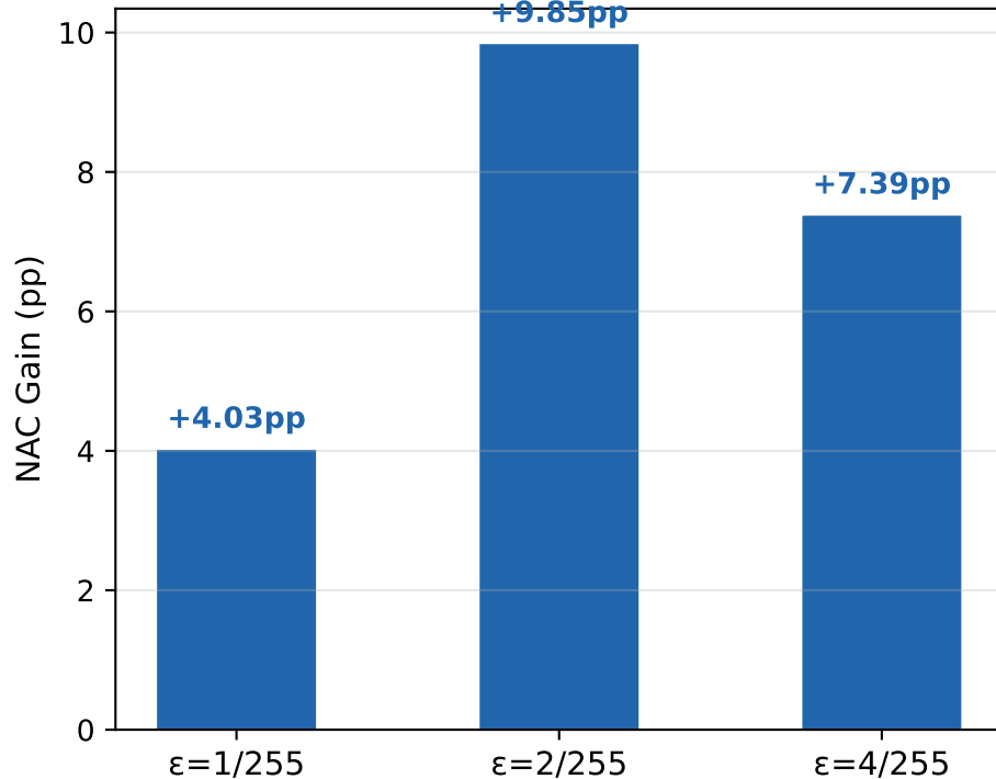
Improvement Margin
