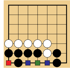
Figure 2.18 – Board with an eye and a union .
