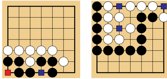
Figure 2.17 – Left: The black group possesses one eye (red) and one union (blue); White must first capture the group on the right (Lemma 2.6.2). Right: The upper-left white group lacks eyes, but shares three unions (blue); Black must capture the neighboring groups in at least two of them before being able to capture it (Lemma 2.6.3).
