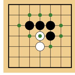
Figure 2.2 – A black group with its adjacencies marked.
