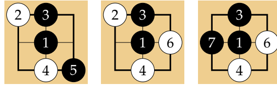
Figure 2.11 – Finished game on a 3 \times 3 board.
