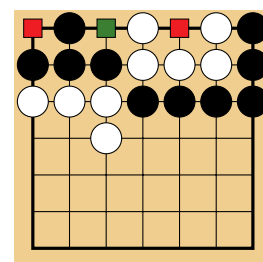
Figure 2.20 – Board with groups in seki .
