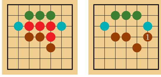
Figure 2.9 – Capture in \text{Go}_4^2 . Brown plays and captures the red group.
