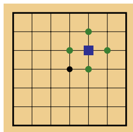
Figure 2.1 – Point (5, 5) in blue, adjacencies in green.
