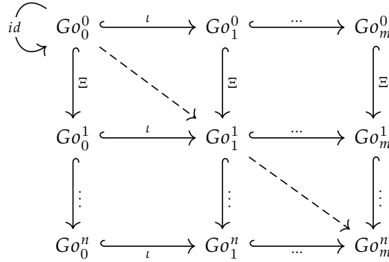
Figure 3.11 – Structure of the family of Go Games. Players are added to the right; the board is expanded downward.
