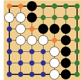
Figure 2.3 – White, black, and neutral territory.
