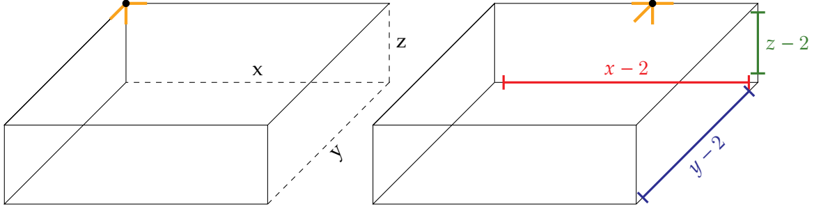
Figure 3.2 – Exterior of the three-dimensional board. A vertex with 3 adjacencies, edges, and a node with 4 adjacencies.
