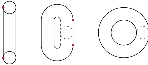
Figure 3.6 – Transition from the cylinder to the torus after joining its opposite faces.
