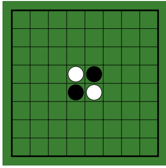
Figure 3.13 – Othello board with its initial position.
