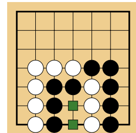
Figure 2.19 – Board with groups in seki .
