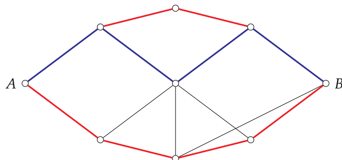
Figure 3.16 – The blue edges belong to Short, the red ones to Cut, and the black ones remain free. The set of blue edges determines a path between the distinguished vertices A and B , so Short wins.
