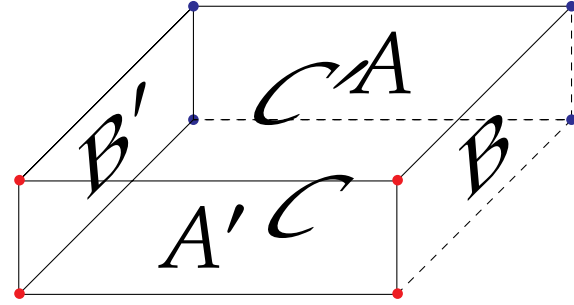
Figure 3.8 – Faces of the Go^3 .
