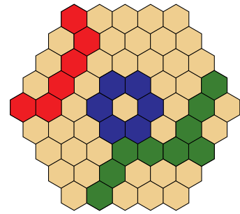
Figure 3.14 – The three winning structures in Havannah: ring , bridge , and fork .
