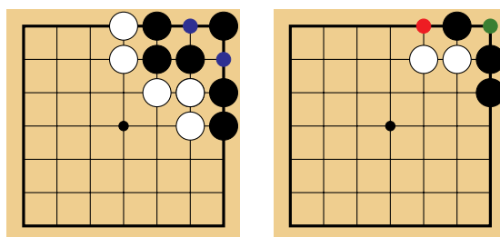
Figure 1.13 – Eyes of a living group (blue). False eye (green). If White plays at the red point, Black will be forced to fill their own eye with a stone, or risk losing it.
