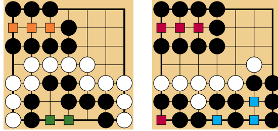
Figure 2.16 – Left: healthy and unhealthy. Right: eyes and unions.
