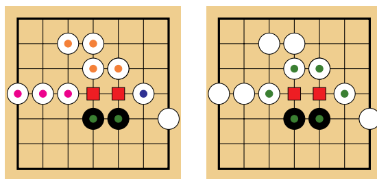
Figure 2.14 – Left: Board with the boundary groups of a Region ; Orange, Magenta, Green, Blue. Right: Adjacencies of a Region .
