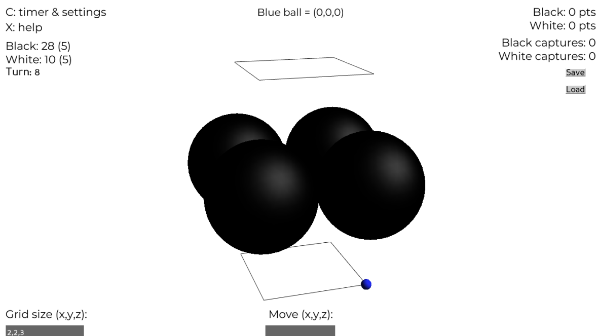
Figure 2.22 – Minimal counterexample to Bai’s result. A two-dimensional black group possessing unconditional life on a 2 \times 2 \times 3 board.
