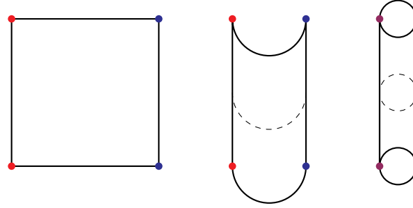
Figure 3.5 – Transition from the plane to a cylinder by joining its opposite sides.
