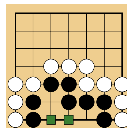
Figure 2.15 – Board with black groups whose controlled region is unhealthy .
