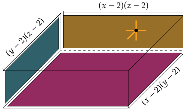
Figure 3.3 – Faces of the three-dimensional board with a node of 5 adjacencies.
