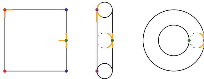
Figure 3.7 – Change in adjacencies from the plane to the torus.
