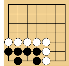
Figure 2.13 – Board with a black group possessing unconditional life.
