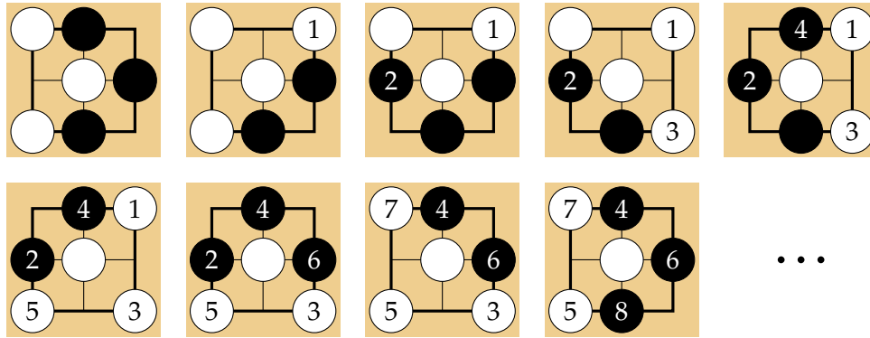
Figure 2.8 – A cycle of length 8 that can be repeated indefinitely in the absence of a Superko rule.
