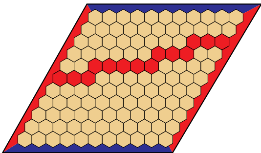
Figure 3.15 – Winning chain connecting two opposite edges.
