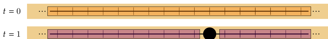
Figure 4.7 – An infinite one dimension and the first turn that shows how a region it's split.
