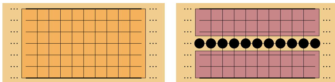
Figure 4.5 – A board where the number of regions (neutral and black) merely grows by one when an infinite group is played.
