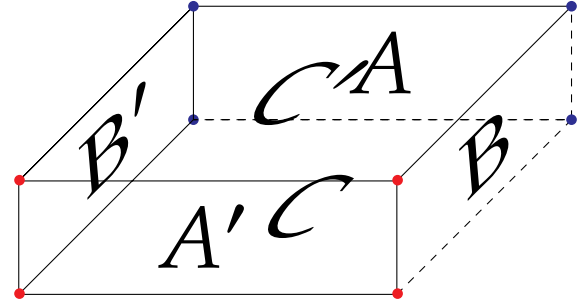
Figure 3.8 – Faces of the Go^3 .
