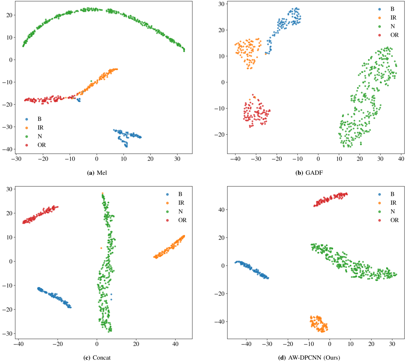
Fig. 10: t-SNE visualization on the CWRU dataset under different fusion strategies. The AW-DPCNN fused representation (d) achieves the most compact intra-class clusters and the clearest inter-class boundaries, consistent with the transformer dataset results.
