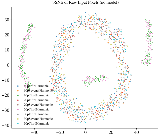
Fig. 11: t-SNE visualization of raw input pixels (PCA 50 \rightarrow t-SNE) for the transformer acoustic dataset. Classes are severely overlapped, demonstrating that raw pixel features are not inherently separable.
