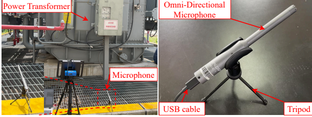
Fig. 5: Experimental platform of acoustic signal acquisition.
