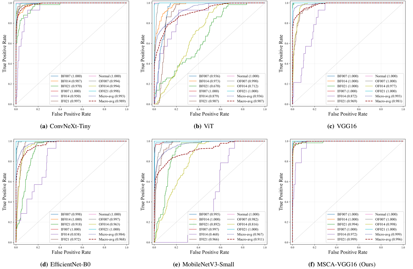
Fig. 7: ROC curves of different backbone networks on the CWUR 12k DE dataset. The proposed MSCA-VGG16 achieves the highest AUC, indicating superior discriminative capability and robustness across classes.
