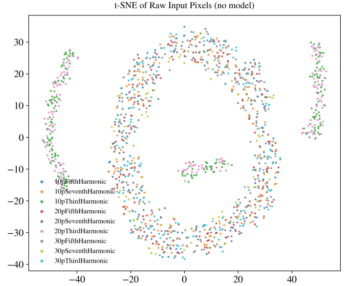
Fig. 11: t-SNE visualization of raw input pixels (PCA 50 \rightarrow t-SNE) for the transformer acoustic dataset. Classes are severely overlapped, demonstrating that raw pixel features are not inherently separable.
