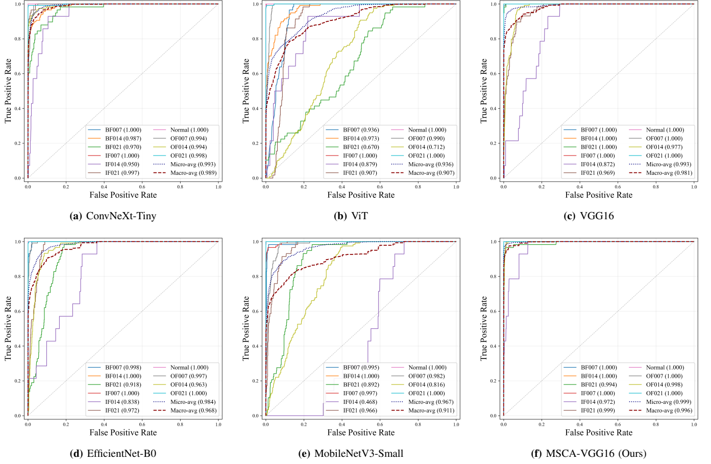
Fig. 10: ROC curves of different backbone networks on the CWRU 12k DE dataset. The proposed MSCA-VGG16 achieves the highest AUC, indicating superior discriminative capability and robustness across classes.
