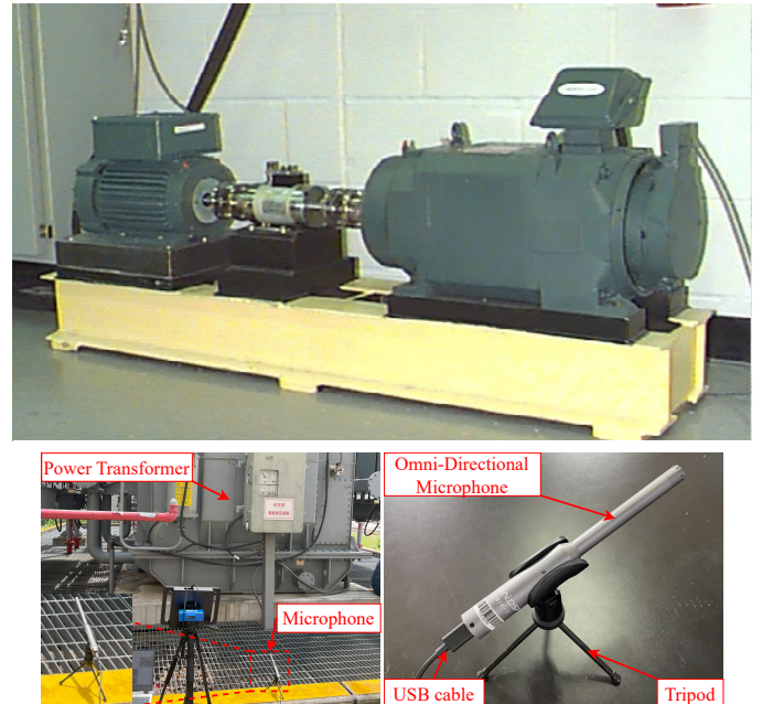
Fig. 5: Test stand of datasets. (a) CWRU bearing dataset. (b) Transformer acoustic dataset.
