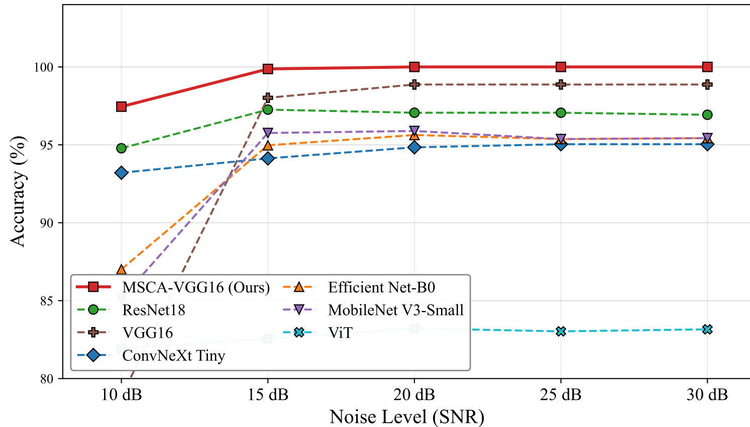
Noise Robustness Comparison — Accuracy vs SNR (Zoomed)
