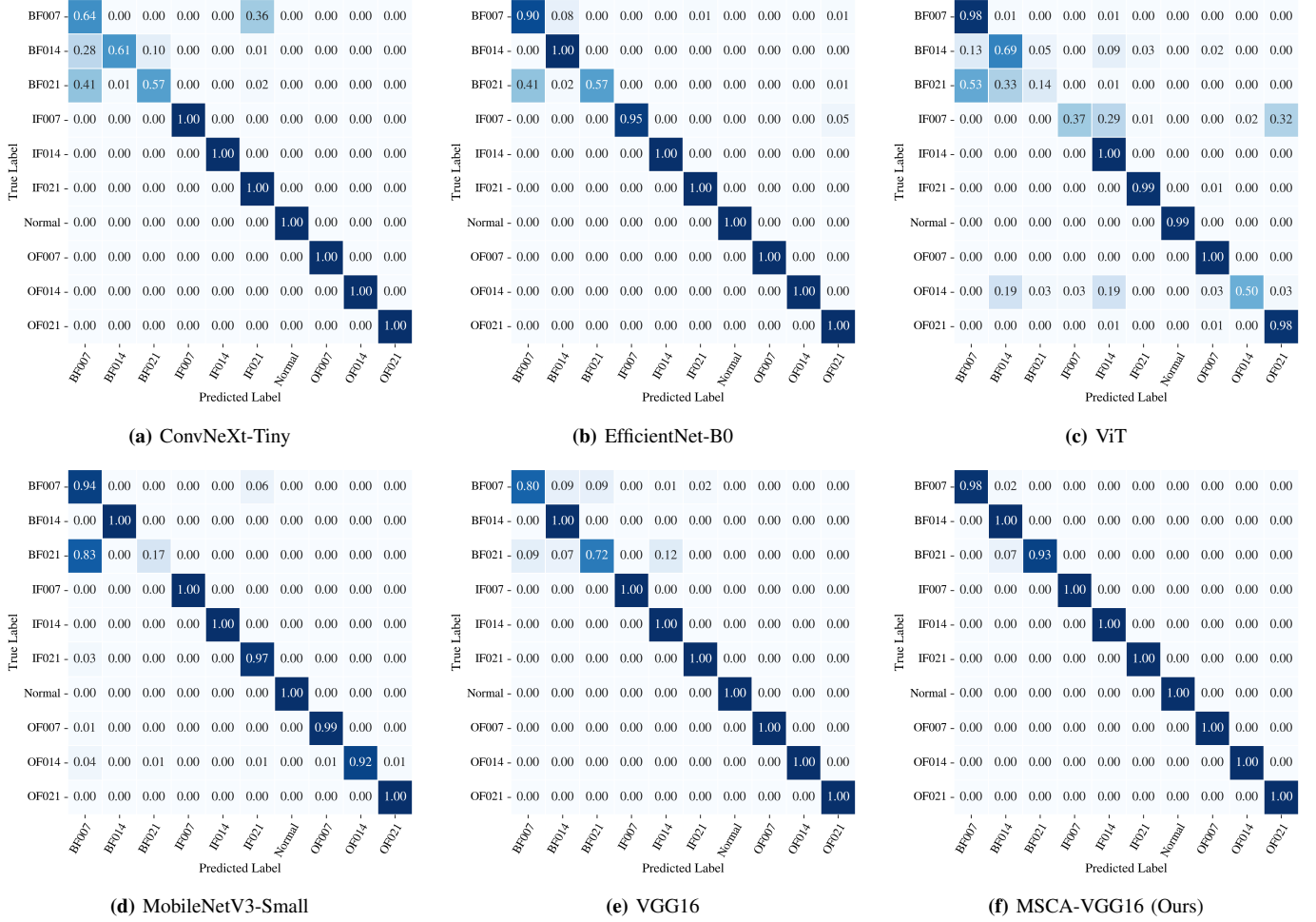
Fig. 8: Confusion matrices of different network backbones trained using the AW-DPCNN fusion representations on the CWRU 12k DE dataset. The proposed MSCA-VGG16 achieves the most accurate classification with significantly reduced inter-class confusion.
