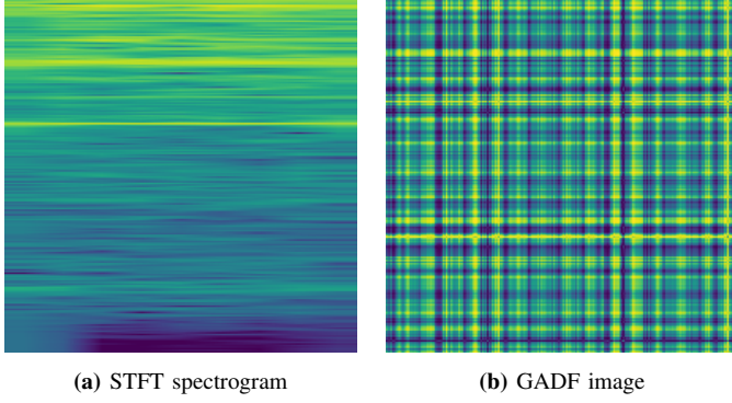
Fig. 2: Vibration signal representations. (a) STFT spectrogram capturing local time–frequency energy distributions. (b) GADF image encoding global temporal correlation structures through pairwise angular relationships.
