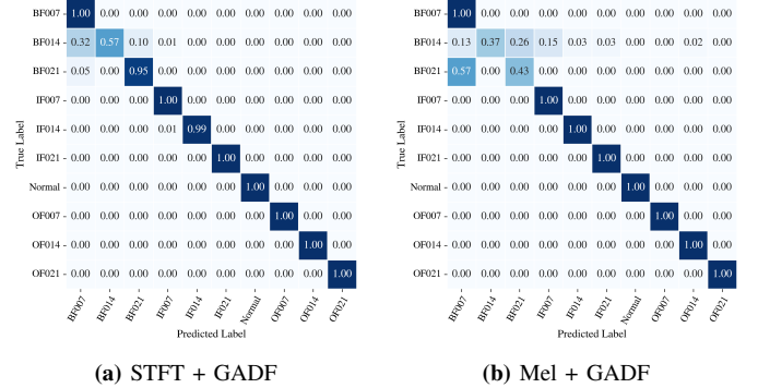
Fig. 7: Confusion matrices of the best-performing (STFT + GADF) and worst-performing (Mel + GADF) representation combinations. STFT + GADF exhibits substantially reduced inter-class confusion, particularly among fault severity levels.
