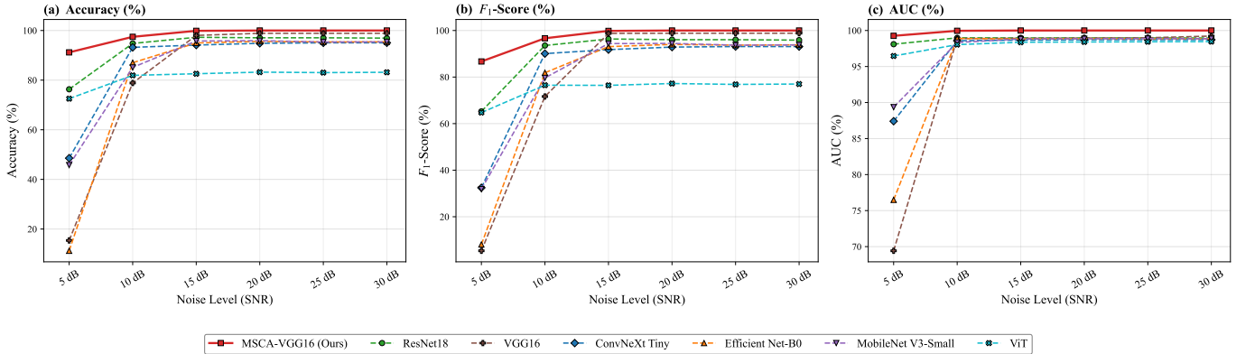
Fig. 11: Noise robustness comparison across seven backbone networks under additive Gaussian noise injection. Panels (a)–(c) report accuracy, F_1 -score, and AUC respectively as functions of SNR level (5.0–30.0 dB). The proposed MSCA-VGG16 achieves 100.0% accuracy at 20.0 dB and maintains 91.2% at 5.0 dB, a degradation of only 8.8%.
