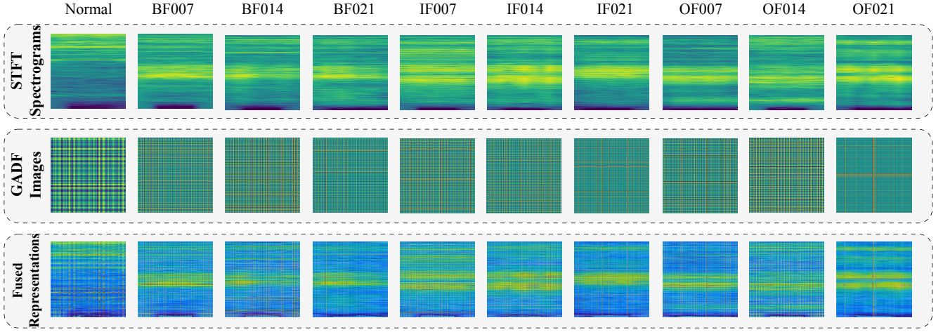
Fig. 5: STFT spectrograms (top), GADF images (middle), and AW-DPCNN fused representations (bottom) for ten bearing conditions.
