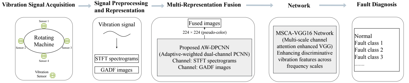
Fig. 1: Overall framework of the proposed vibration signal fault diagnosis method. The vibration signal is first converted into STFT spectrograms and GADF images. These heterogeneous representations are then adaptively fused through the proposed AW-DPCNN mechanism. Finally, the fused features are fed into the MSCA-VGG16 network for fault classification.
