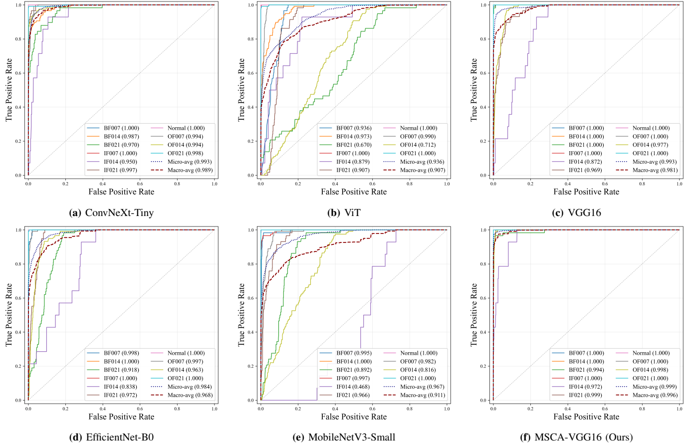
Fig. 9: ROC curves of different backbone networks on the CWRU 12k DE dataset. The proposed MSCA-VGG16 achieves higher AUC on most classes, indicating superior discriminative capability and robustness across classes.
