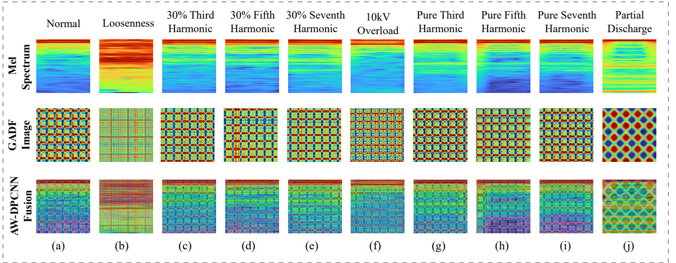
Fig. 5: Visualization of Mel spectrograms, GADF images, and adaptively fused representations generated by the proposed AW-DPCNN under different transformer operating conditions. (a) Normal, (b) Loosen, (c) 30% Third Harmonic Distortion, (d) 30% Fifth Harmonic Distortion, (e) 30% Seventh Harmonic Distortion, (f) 10kV Overload, (g) Pure Third Harmonic, (h) Pure Fifth Harmonic, (i) Pure Seventh Harmonic, and (j) Partial Discharge.
