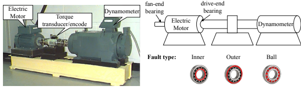
Figure 6: CWRU bearing test stand. Vibration signals were collected from accelerometers at the drive-end and fan-end positions under four operating loads (0–3 hp).
