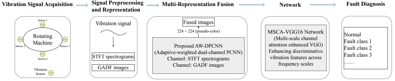
Figure 1: Overall framework of the proposed vibration signal fault diagnosis method. The vibration signal is first converted into STFT spectrograms and GADF images. These heterogeneous representations are then adaptively fused through the proposed AW-DPCNN mechanism. Finally, the fused features are fed into the MSCA-VGG16 network for fault classification.
