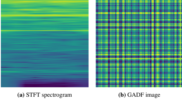
Figure 2: Vibration signal representations. (a) STFT spectrogram capturing local time–frequency energy distributions. (b) GADF image encoding global temporal correlation structures through pairwise angular relationships.
