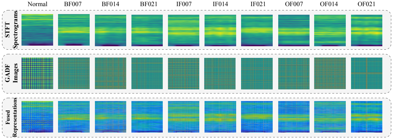
Figure 5: STFT spectrograms (top), GADF images (middle), and AW-DPCNN fused representations (bottom) for ten bearing conditions.
