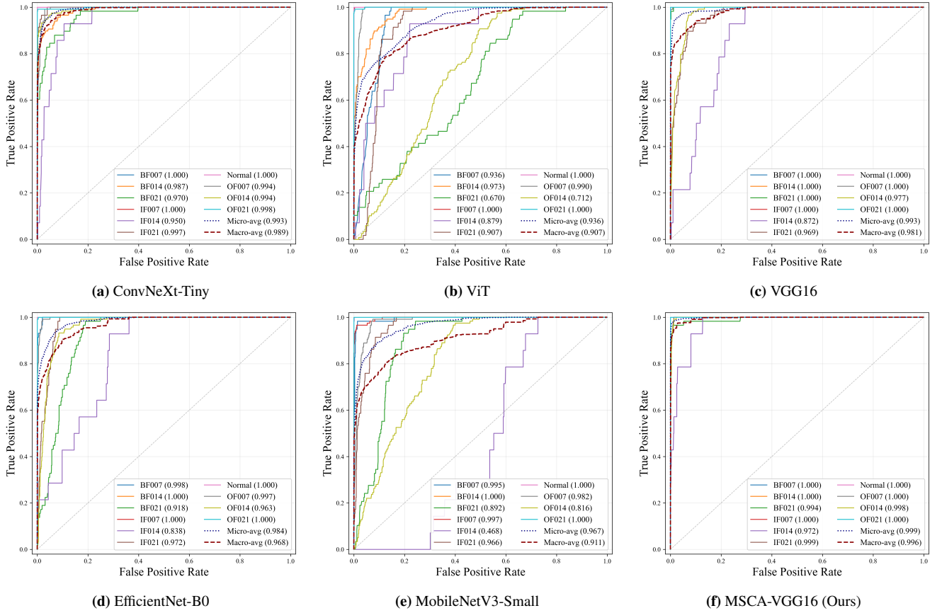
Figure 9: ROC curves of different backbone networks on the CWRU 12k DE dataset. The proposed MSCA-VGG16 achieves higher AUC on most classes, indicating superior discriminative capability and robustness across classes.
