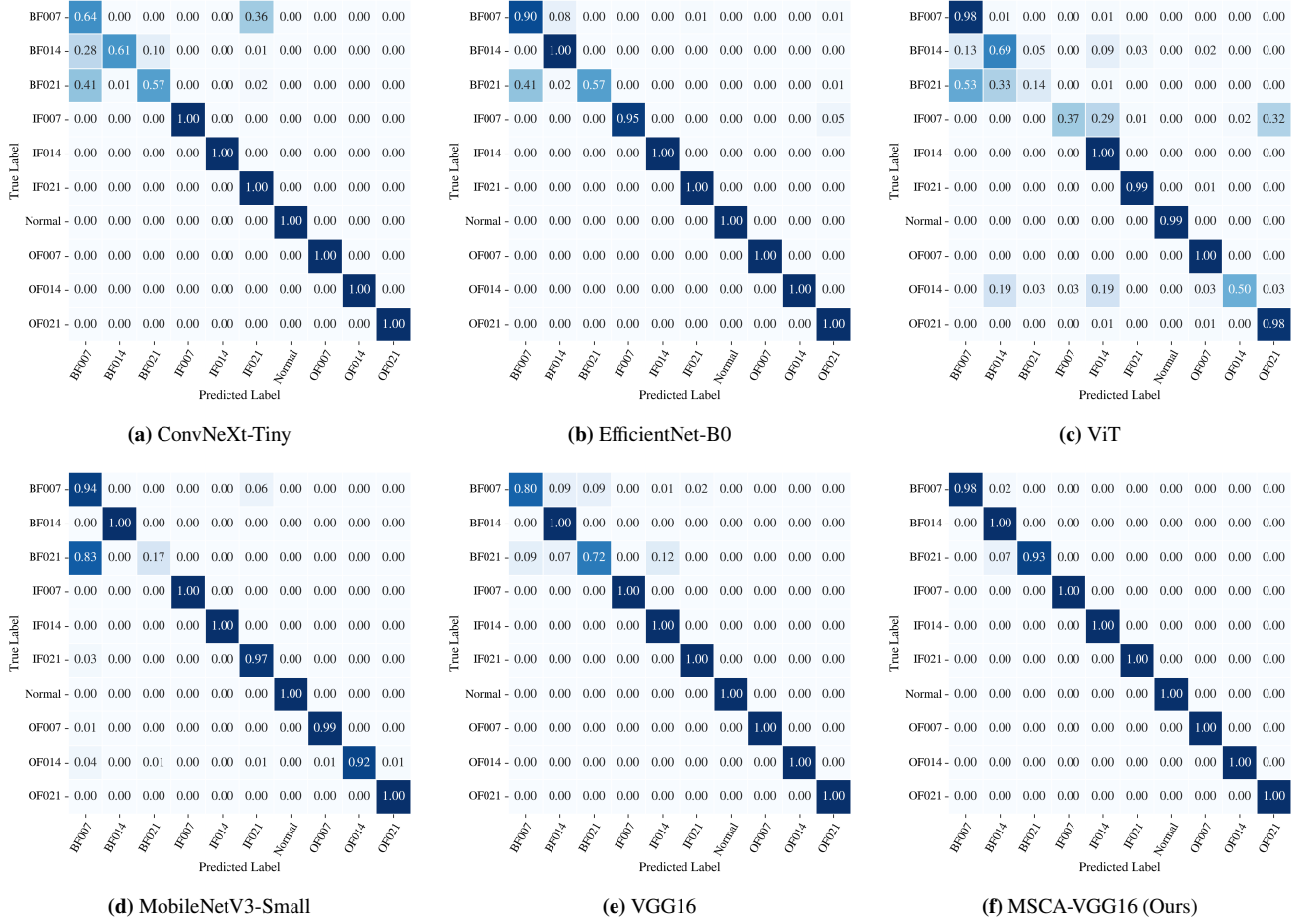
Figure 8: Confusion matrices of different network backbones trained using the AW-DPCNN fusion representations on the CWRU 12k DE dataset. The proposed MSCA-VGG16 achieves the most accurate classification with significantly reduced inter-class confusion.
