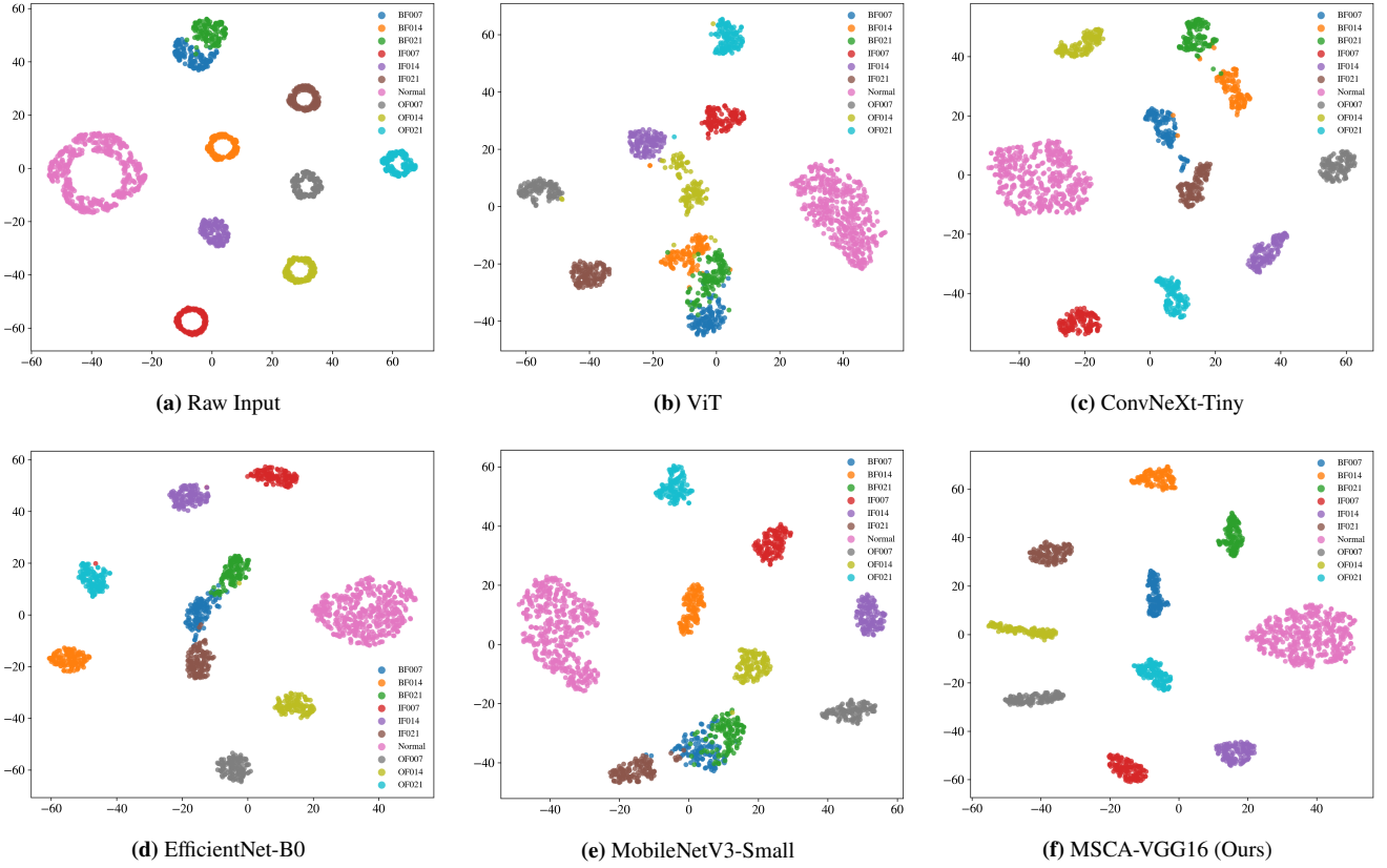
Figure 10: t-SNE feature visualization of different backbone networks on the CWRU 12k DE bearing test set. The proposed MSCA-VGG16 produces the most compact and well-separated clusters, indicating superior discriminative representation learning.
