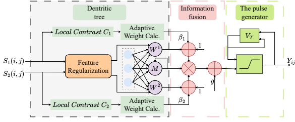
Figure 3: Architecture of the proposed adaptive weighted dual-channel PCNN (AW-DPCNN) for multi-representation signal fusion. The mechanism comprises contrast-guided adaptive weighting, dual-channel PCNN with representation-specific convolutional kernels, and iterative pulse-coupled dynamics for feature reinforcement.
