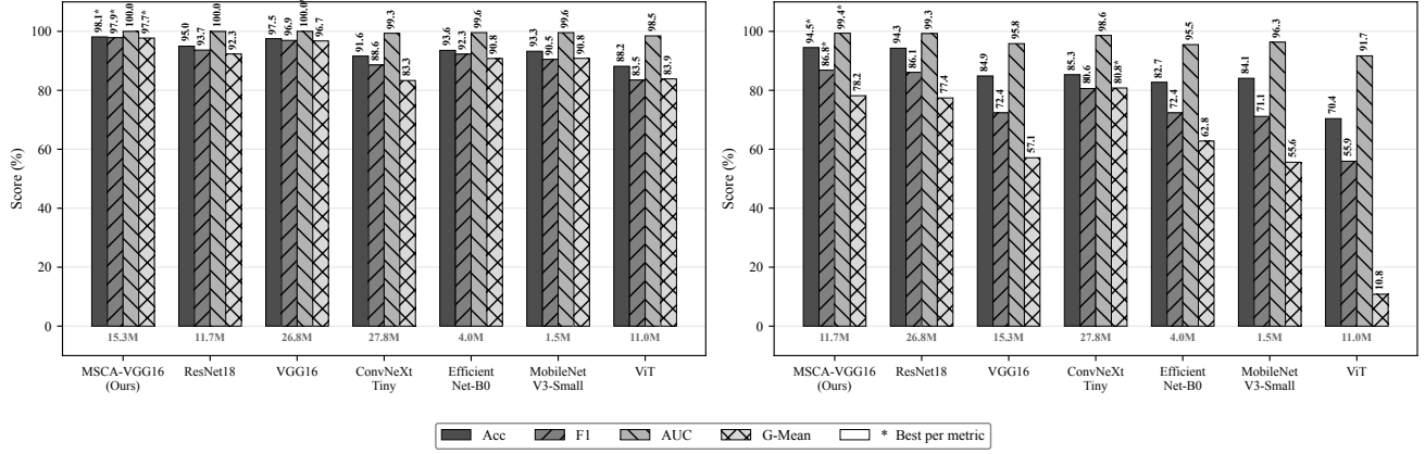
Figure 12: Generalization validation across seven backbone networks on the CWRU 12k FE (left) and 48k DE (right) datasets. Best per metric marked with an asterisk. MSCA-VGG16 achieves the highest or competitive scores across all metrics on both datasets, with the most pronounced advantages in F1-score and G-mean under cross-sampling-rate conditions.
