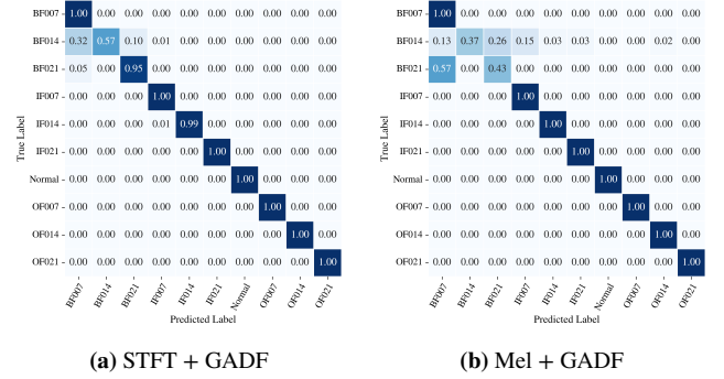
Figure 7: Confusion matrices of the best-performing (STFT + GADF) and worst-performing (Mel + GADF) representation combinations. STFT + GADF exhibits substantially reduced inter-class confusion, particularly among fault severity levels.
