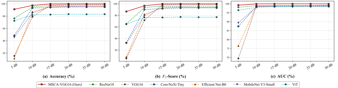
Figure 11: Noise robustness comparison across seven backbone networks under additive Gaussian noise injection. Panels (a)–(c) report accuracy, F_1 -score, and AUC respectively as functions of SNR level (5.0–30.0 dB). The proposed MSCA-VGG16 achieves 100.0% accuracy at 20.0 dB and maintains 91.2% at 5.0 dB, a degradation of only 8.8%.
