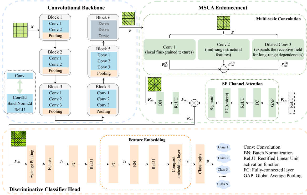
Figure 4: Architecture of the proposed MSCA-VGG16 network. The fused AW-DPCNN image is processed by a VGG16-BN backbone, followed by multi-scale convolution (MS), squeeze-and-excitation channel attention (SE), and a compact embedding head (EH) for fault classification.
