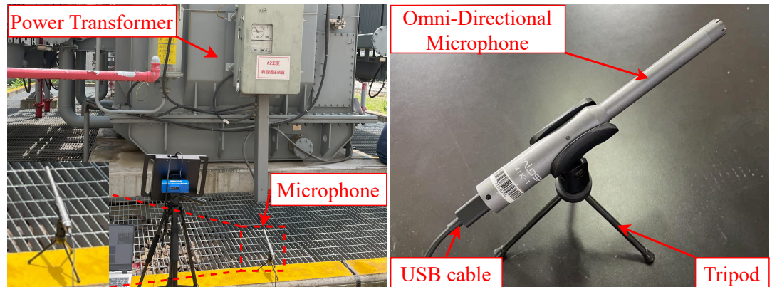
Figure 5: Experimental platform of acoustic signal acquisition.
